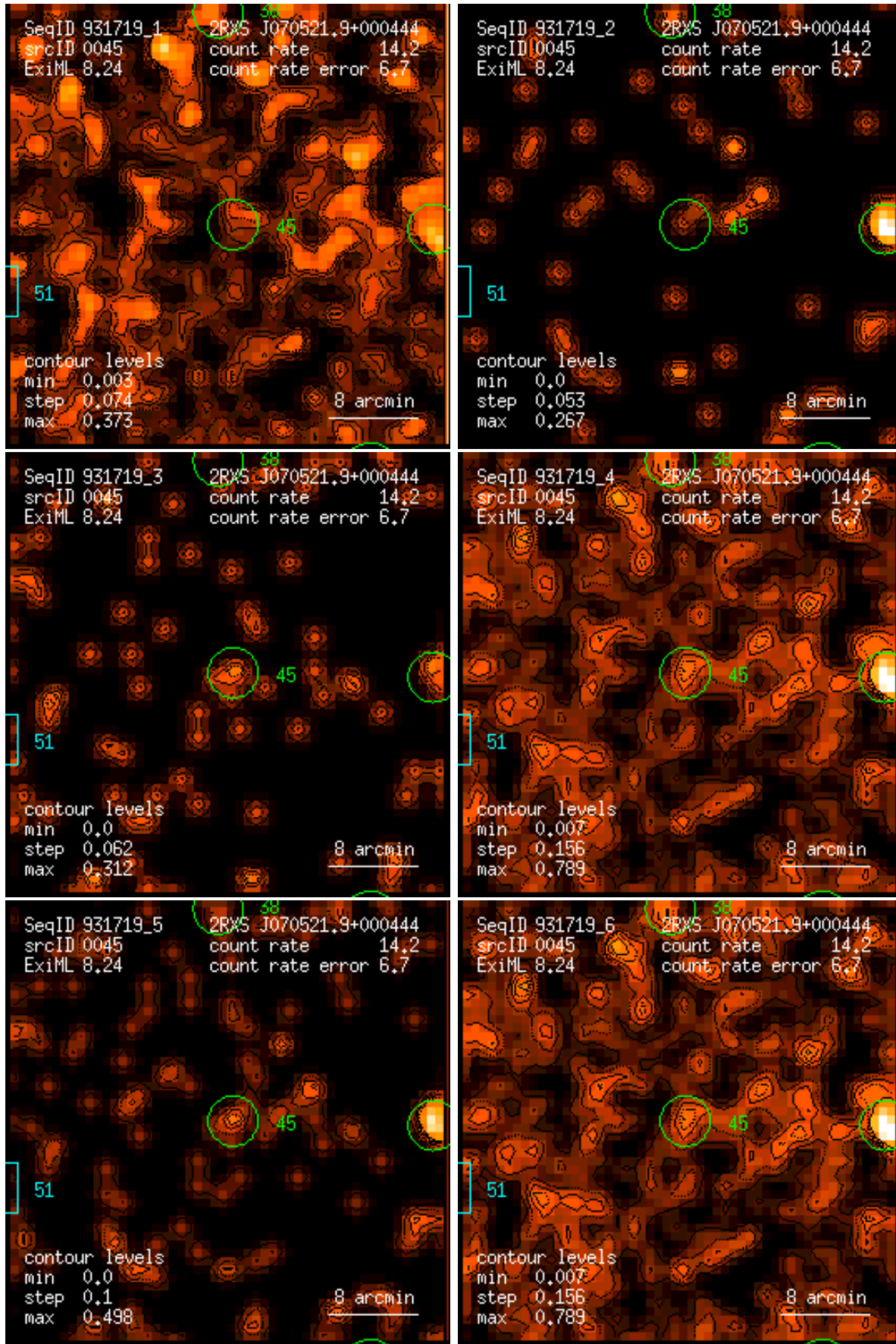
Figure 45: RASS 931719: detection 0045: band rate images, Gaussian filter: (1) PSPC channels 11 – 41, (2) 52 – 90, (3) 91 – 201, (4) 11 – 235, (5) 52 – 201, (6) 11 – 201. Broad band rates in counts/ks. Band rate contour levels in counts/ks/arcmin 2 .
