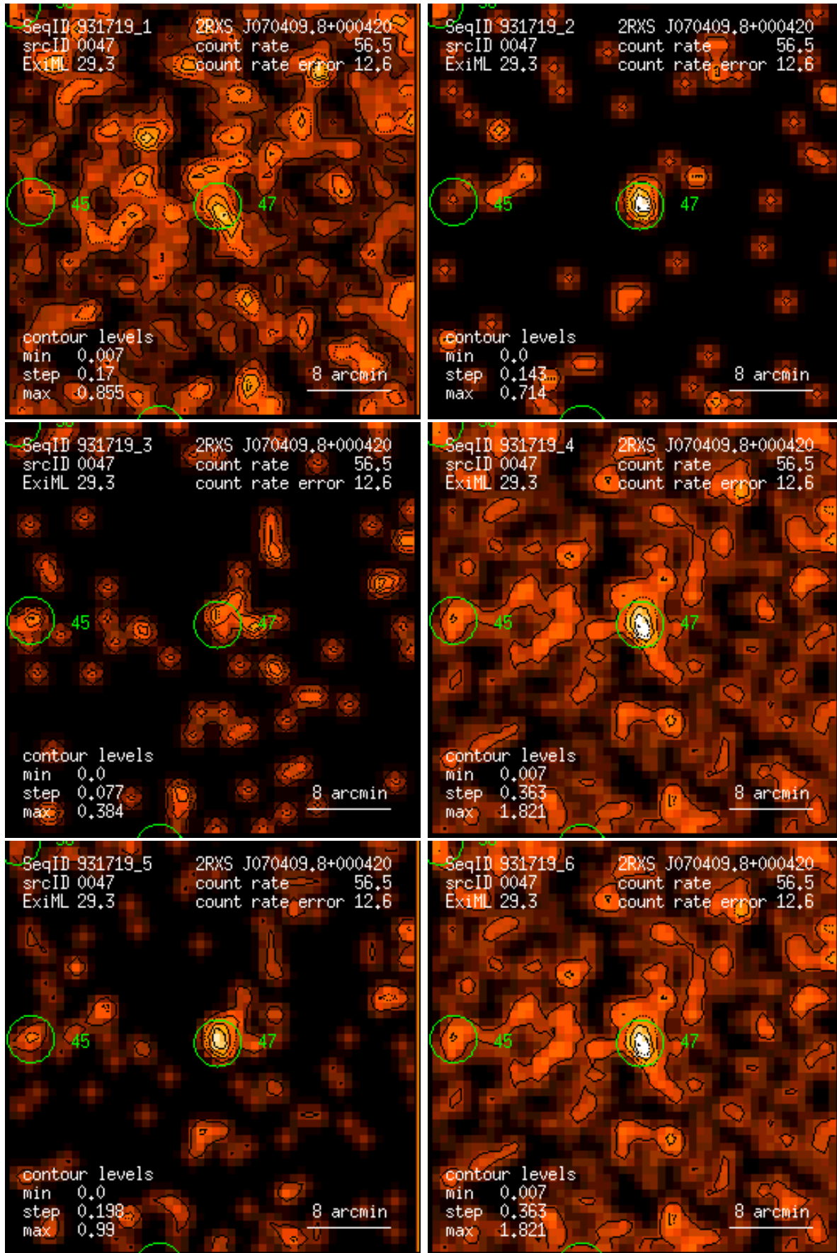
Figure 47: RASS 931719: detection 0047: band rate images, Gaussian filter: (1) PSPC channels 11 – 41, (2) 52 – 90, (3) 91 – 201, (4) 11 – 235, (5) 52 – 201, (6) 11 – 201. Broad band rates in counts/ks. Band rate contour levels in counts/ks/arcmin 2 .
