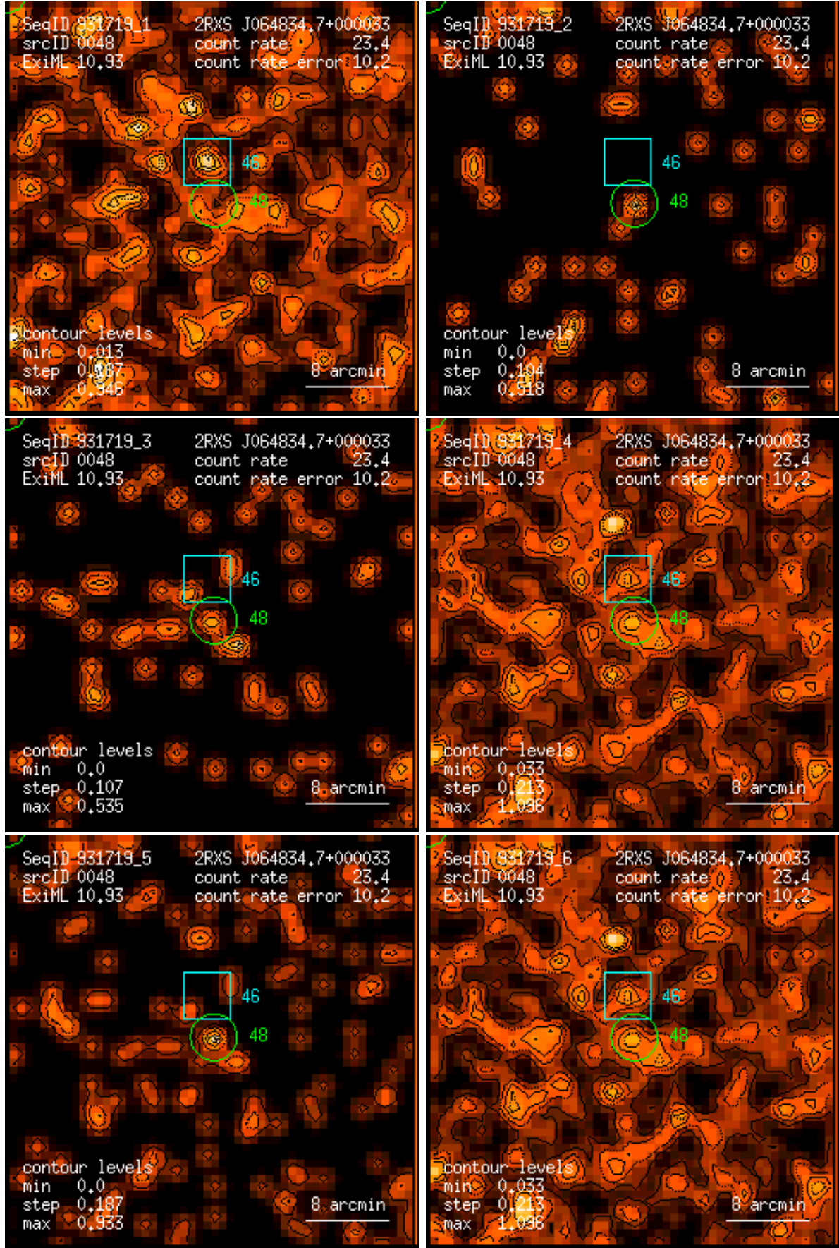
Figure 48: RASS 931719: detection 0048: band rate images, Gaussian filter: (1) PSPC channels 11 – 41, (2) 52 – 90, (3) 91 – 201, (4) 11 – 235, (5) 52 – 201, (6) 11 – 201. Broad band rates in counts/ks. Band rate contour levels in counts/ks/arcmin 2 .
