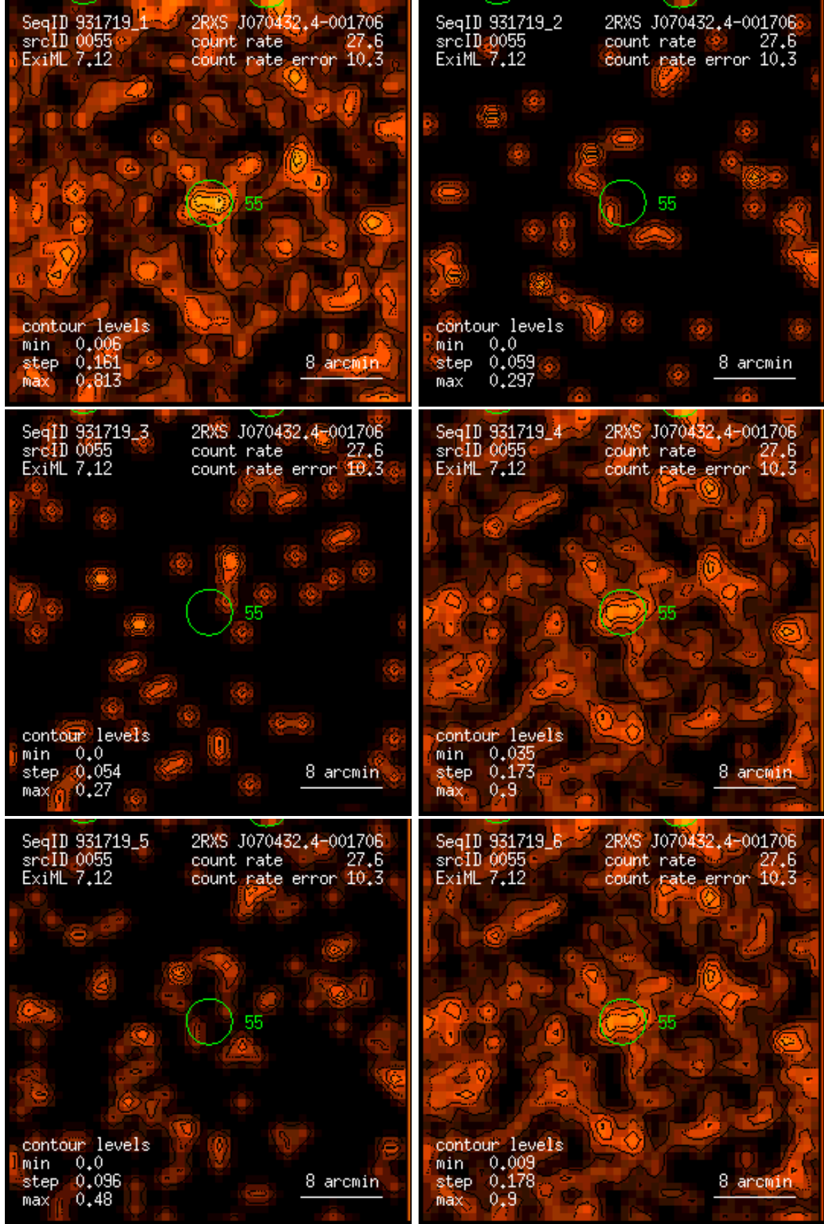
Figure 55: RASS 931719: detection 0055: band rate images, Gaussian filter: (1) PSPC channels 11 – 41, (2) 52 – 90, (3) 91 – 201, (4) 11 – 235, (5) 52 – 201, (6) 11 – 201. Broad band rates in counts/ks. Band rate contour levels in counts/ks/arcmin 2 .
