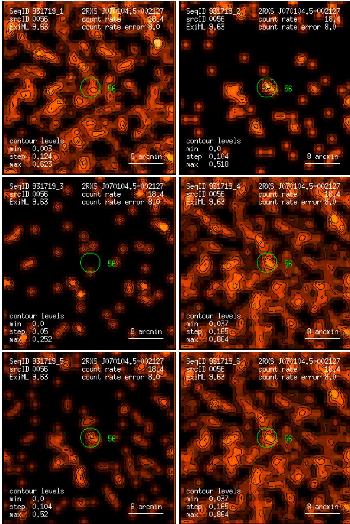
Figure 56: RASS 931719: detection 0056: band rate images, Gaussian filter: (1) PSPC channels 11 – 41, (2) 52 – 90, (3) 91 – 201, (4) 11 – 235, (5) 52 – 201, (6) 11 – 201. Broad band rates in counts/ks. Band rate contour levels in counts/ks/arcmin 2 .
