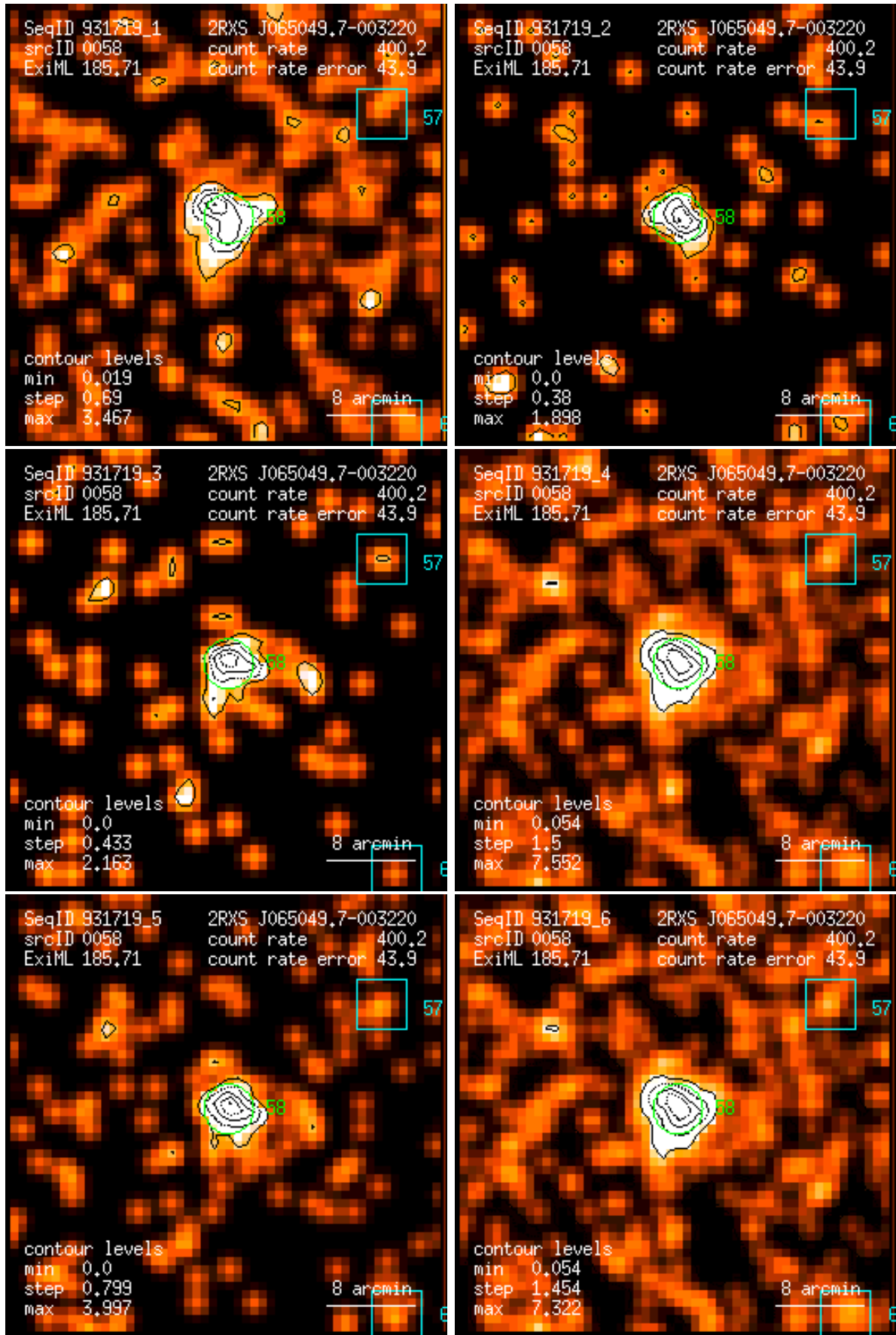
Figure 58: RASS 931719: detection 0058: band rate images, Gaussian filter: (1) PSPC channels 11 – 41, (2) 52 – 90, (3) 91 – 201, (4) 11 – 235, (5) 52 – 201, (6) 11 – 201. Broad band rates in counts/ks. Band rate contour levels in counts/ks/arcmin 2 .
