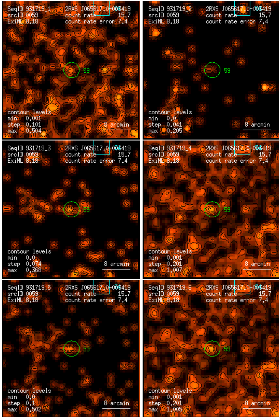
Figure 59: RASS 931719: detection 0059: band rate images, Gaussian filter: (1) PSPC channels 11 – 41, (2) 52 – 90, (3) 91 – 201, (4) 11 – 235, (5) 52 – 201, (6) 11 – 201. Broad band rates in counts/ks. Band rate contour levels in counts/ks/arcmin 2 .
