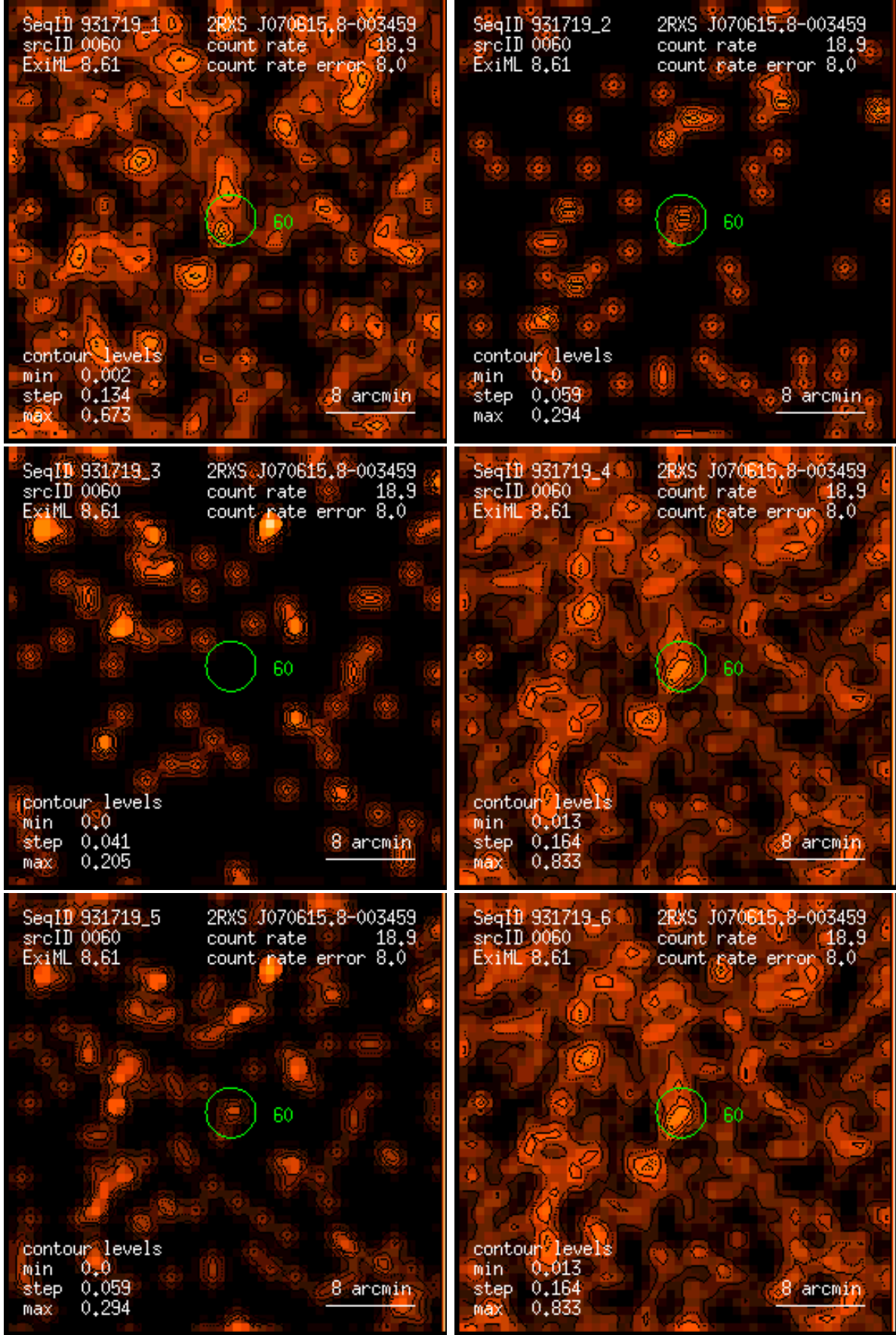
Figure 60: RASS 931719: detection 0060: band rate images, Gaussian filter: (1) PSPC channels 11 – 41, (2) 52 – 90, (3) 91 – 201, (4) 11 – 235, (5) 52 – 201, (6) 11 – 201. Broad band rates in counts/ks. Band rate contour levels in counts/ks/arcmin 2 .
