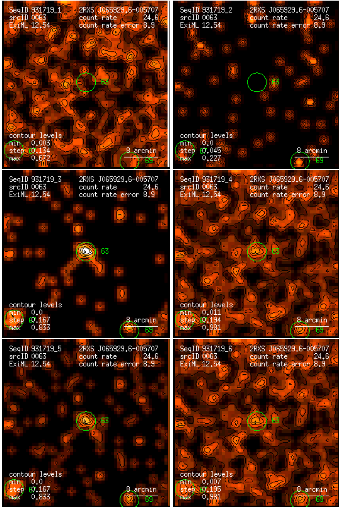
Figure 63: RASS 931719: detection 0063: band rate images, Gaussian filter: (1) PSPC channels 11 – 41, (2) 52 – 90, (3) 91 – 201, (4) 11 – 235, (5) 52 – 201, (6) 11 – 201. Broad band rates in counts/ks. Band rate contour levels in counts/ks/arcmin 2 .
