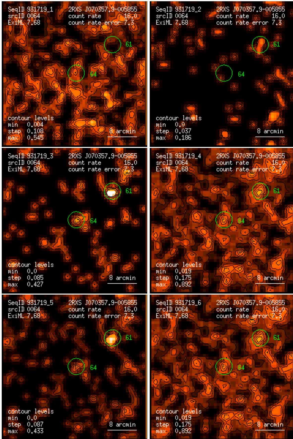
Figure 64: RASS 931719: detection 0064: band rate images, Gaussian filter: (1) PSPC channels 11 – 41, (2) 52 – 90, (3) 91 – 201, (4) 11 – 235, (5) 52 – 201, (6) 11 – 201. Broad band rates in counts/ks. Band rate contour levels in counts/ks/arcmin 2 .
