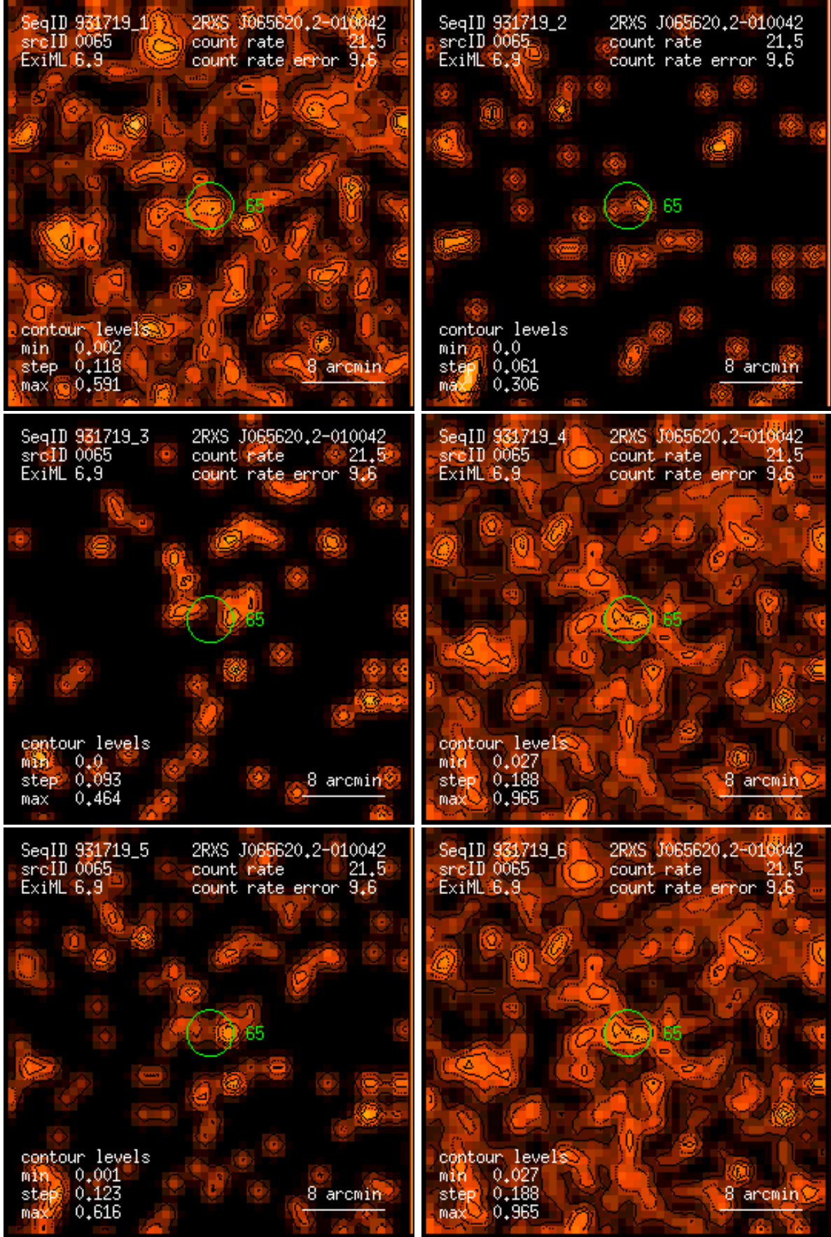
Figure 65: RASS 931719: detection 0065: band rate images, Gaussian filter: (1) PSPC channels 11 – 41, (2) 52 – 90, (3) 91 – 201, (4) 11 – 235, (5) 52 – 201, (6) 11 – 201. Broad band rates in counts/ks. Band rate contour levels in counts/ks/arcmin 2 .
