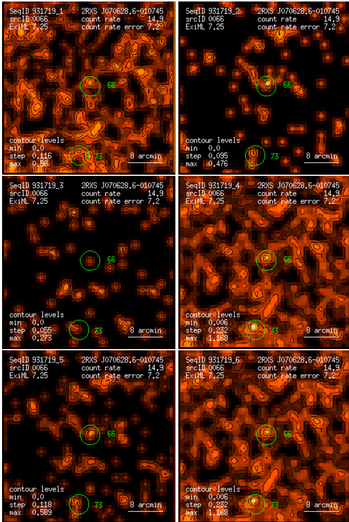
Figure 66: RASS 931719: detection 0066: band rate images, Gaussian filter: (1) PSPC channels 11 – 41, (2) 52 – 90, (3) 91 – 201, (4) 11 – 235, (5) 52 – 201, (6) 11 – 201. Broad band rates in counts/ks. Band rate contour levels in counts/ks/arcmin 2 .
