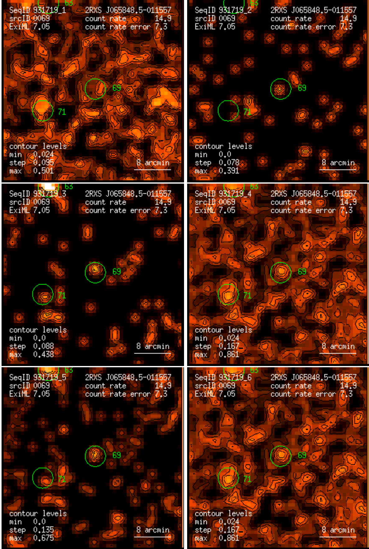
Figure 69: RASS 931719: detection 0069: band rate images, Gaussian filter: (1) PSPC channels 11 – 41, (2) 52 – 90, (3) 91 – 201, (4) 11 – 235, (5) 52 – 201, (6) 11 – 201. Broad band rates in counts/ks. Band rate contour levels in counts/ks/arcmin 2 .
