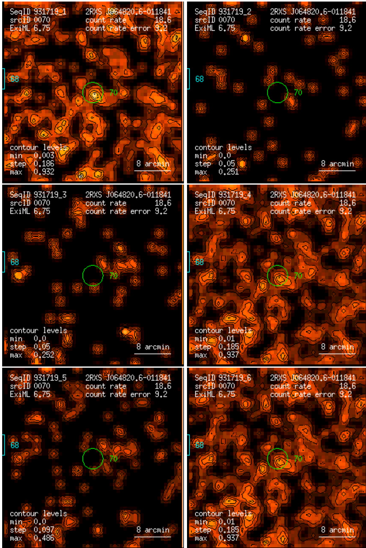
Figure 70: RASS 931719: detection 0070: band rate images, Gaussian filter: (1) PSPC channels 11 – 41, (2) 52 – 90, (3) 91 – 201, (4) 11 – 235, (5) 52 – 201, (6) 11 – 201. Broad band rates in counts/ks. Band rate contour levels in counts/ks/arcmin 2 .
