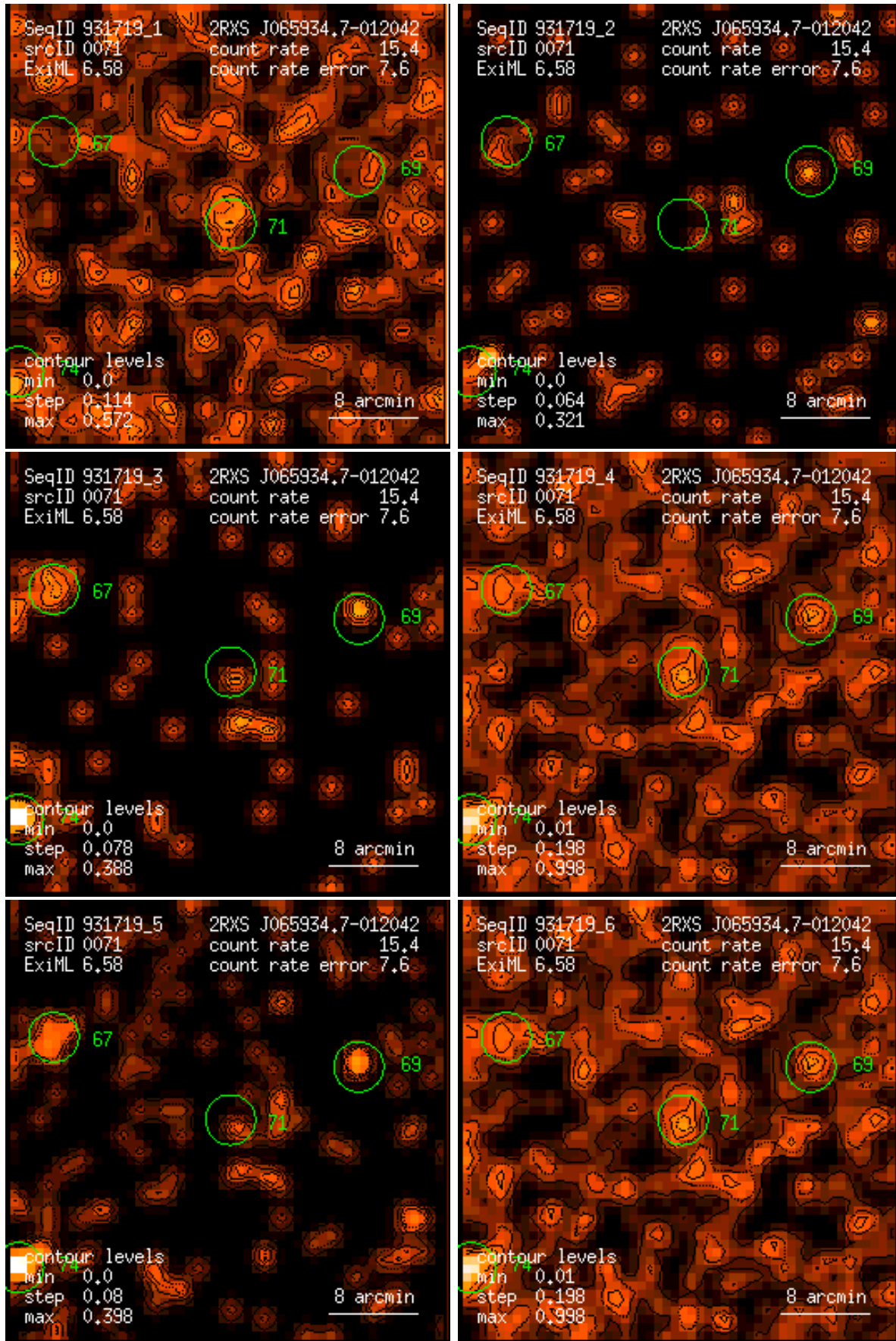
Figure 71: RASS 931719: detection 0071: band rate images, Gaussian filter: (1) PSPC channels 11 – 41, (2) 52 – 90, (3) 91 – 201, (4) 11 – 235, (5) 52 – 201, (6) 11 – 201. Broad band rates in counts/ks. Band rate contour levels in counts/ks/arcmin 2 .
