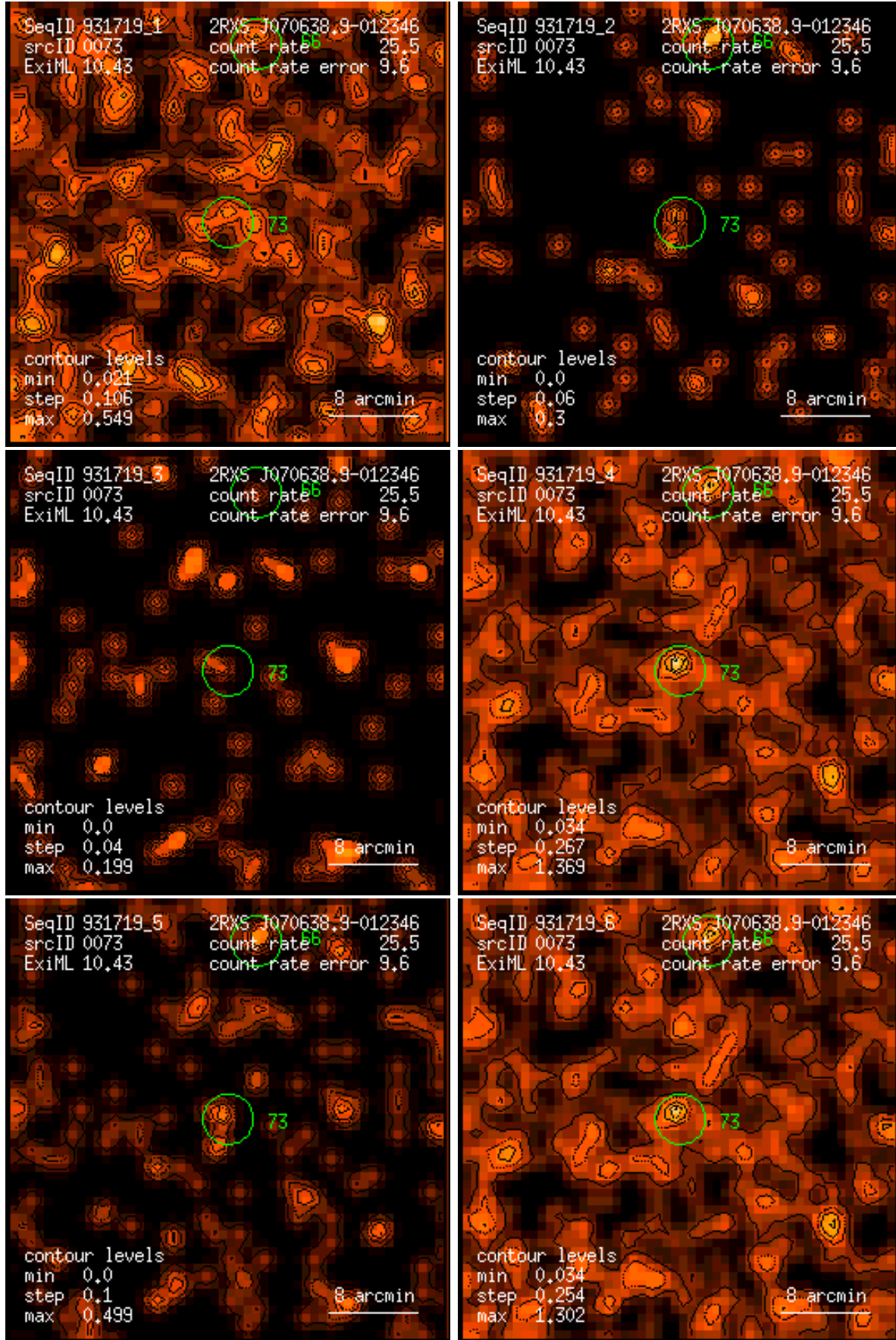
Figure 73: RASS 931719: detection 0073: band rate images, Gaussian filter: (1) PSPC channels 11 – 41, (2) 52 – 90, (3) 91 – 201, (4) 11 – 235, (5) 52 – 201, (6) 11 – 201. Broad band rates in counts/ks. Band rate contour levels in counts/ks/arcmin 2 .
