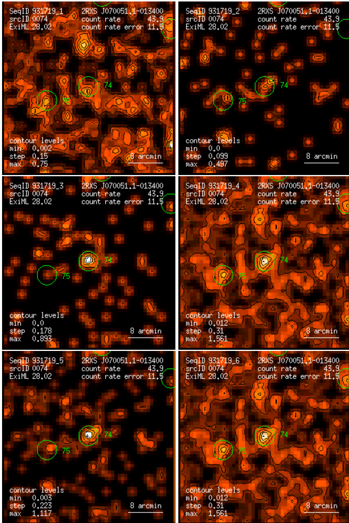
Figure 74: RASS 931719: detection 0074: band rate images, Gaussian filter: (1) PSPC channels 11 – 41, (2) 52 – 90, (3) 91 – 201, (4) 11 – 235, (5) 52 – 201, (6) 11 – 201. Broad band rates in counts/ks. Band rate contour levels in counts/ks/arcmin 2 .
