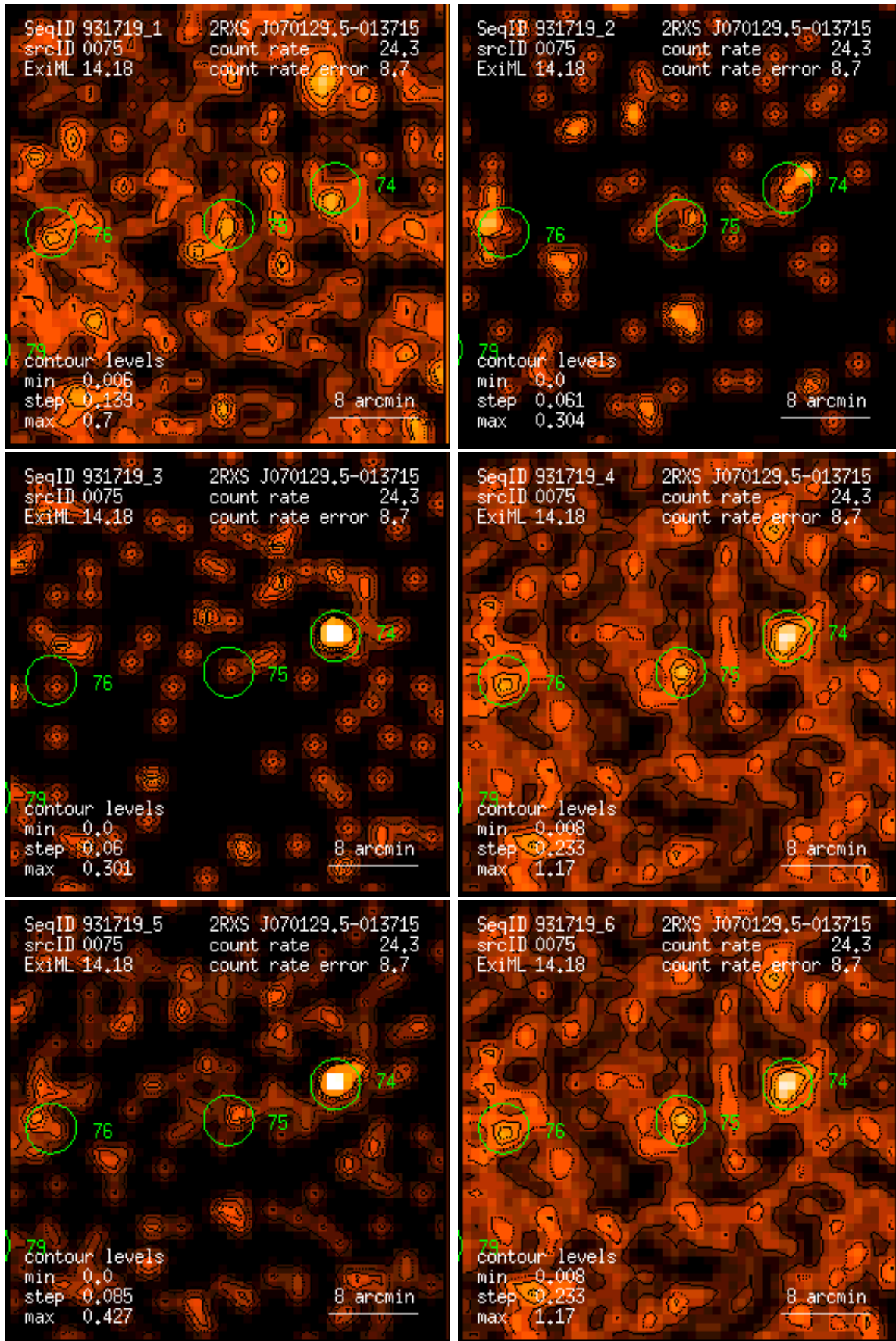
Figure 75: RASS 931719: detection 0075: band rate images, Gaussian filter: (1) PSPC channels 11 – 41, (2) 52 – 90, (3) 91 – 201, (4) 11 – 235, (5) 52 – 201, (6) 11 – 201. Broad band rates in counts/ks. Band rate contour levels in counts/ks/arcmin 2 .
