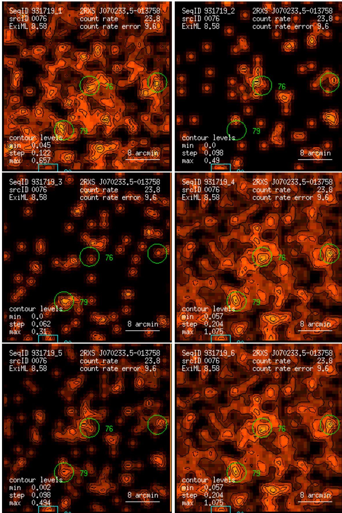
Figure 76: RASS 931719: detection 0076: band rate images, Gaussian filter: (1) PSPC channels 11 – 41, (2) 52 – 90, (3) 91 – 201, (4) 11 – 235, (5) 52 – 201, (6) 11 – 201. Broad band rates in counts/ks. Band rate contour levels in counts/ks/arcmin 2 .
