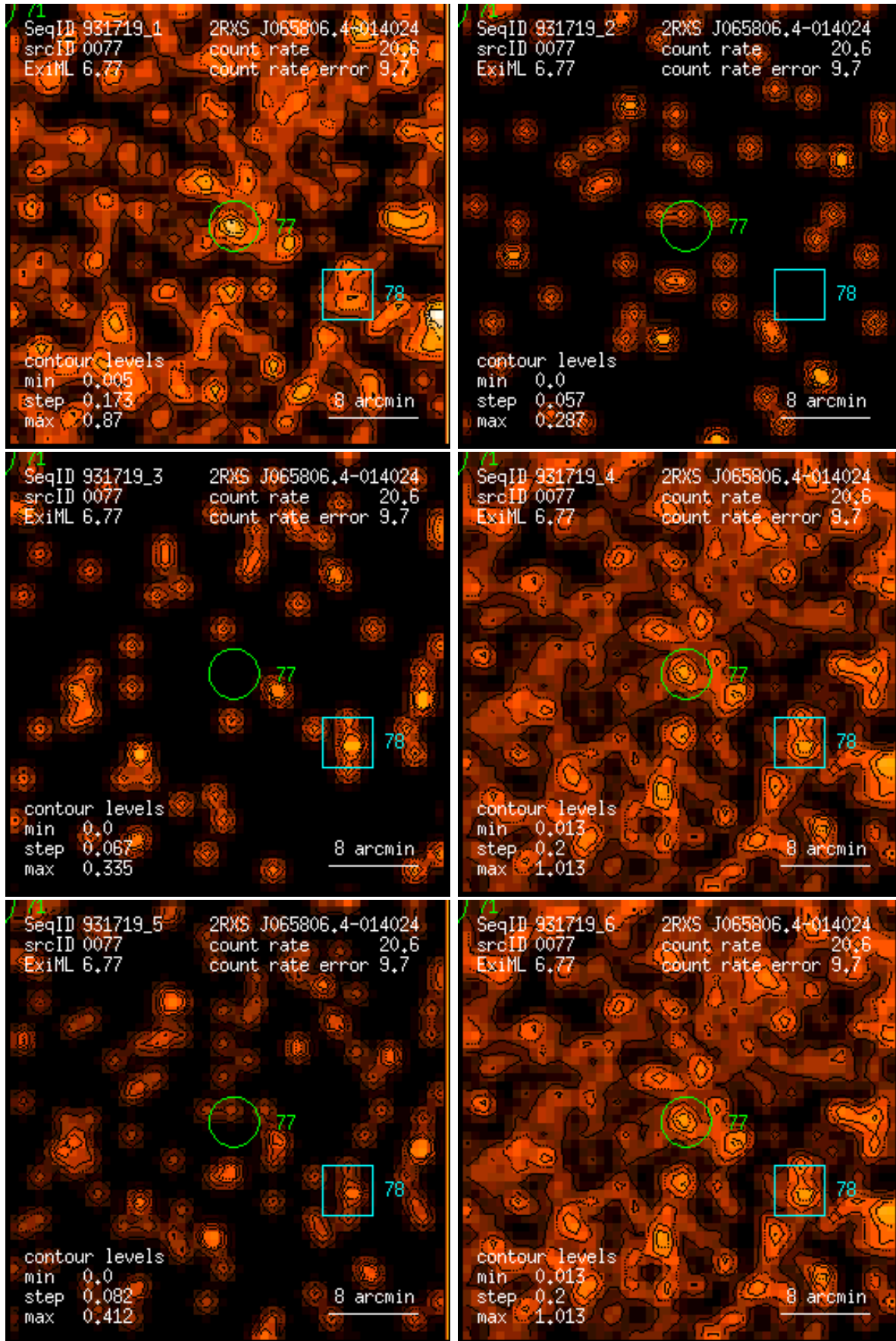
Figure 77: RASS 931719: detection 0077: band rate images, Gaussian filter: (1) PSPC channels 11 – 41, (2) 52 – 90, (3) 91 – 201, (4) 11 – 235, (5) 52 – 201, (6) 11 – 201. Broad band rates in counts/ks. Band rate contour levels in counts/ks/arcmin 2 .
