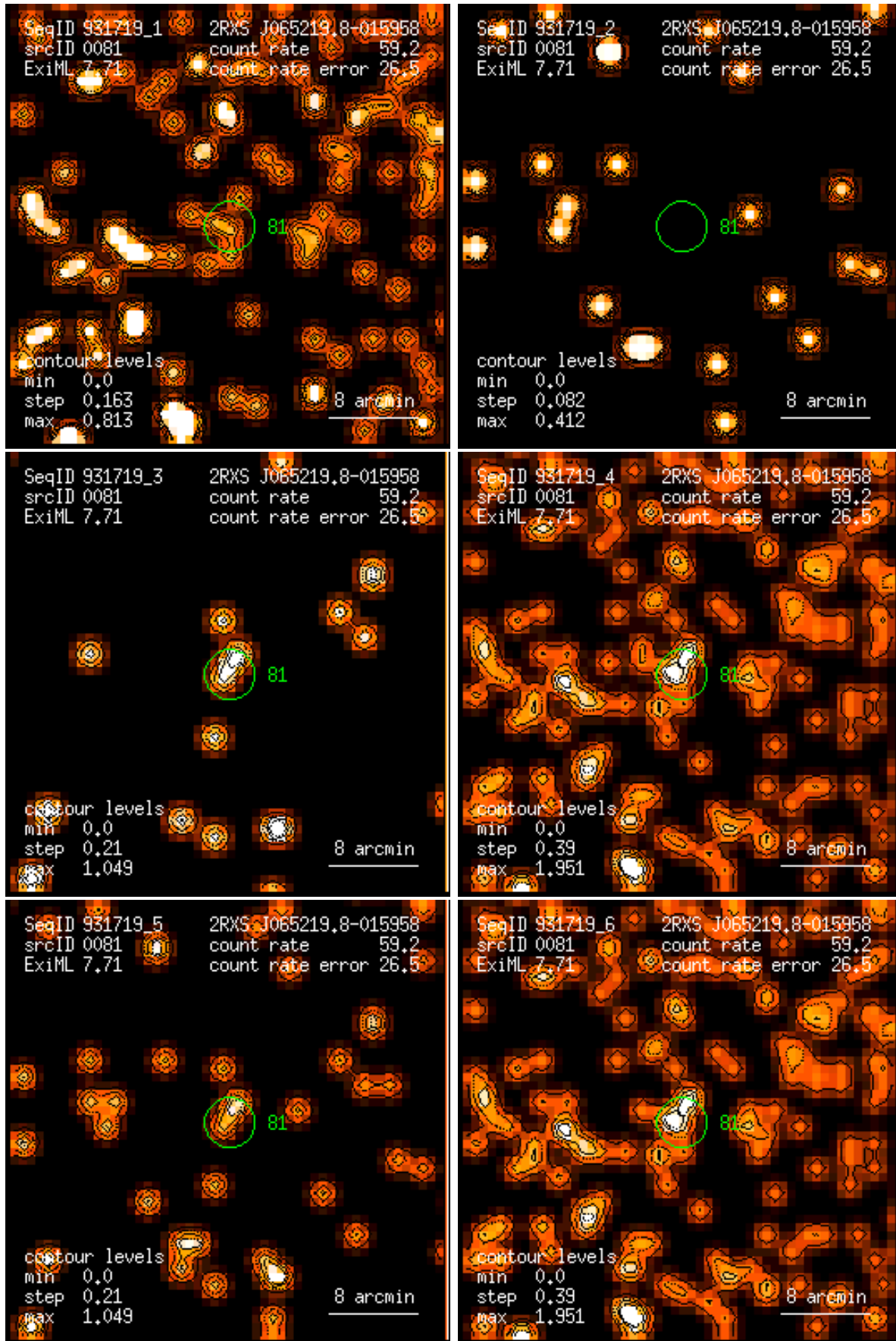
Figure 81: RASS 931719: detection 0081: band rate images, Gaussian filter: (1) PSPC channels 11 – 41, (2) 52 – 90, (3) 91 – 201, (4) 11 – 235, (5) 52 – 201, (6) 11 – 201. Broad band rates in counts/ks. Band rate contour levels in counts/ks/arcmin 2 .
