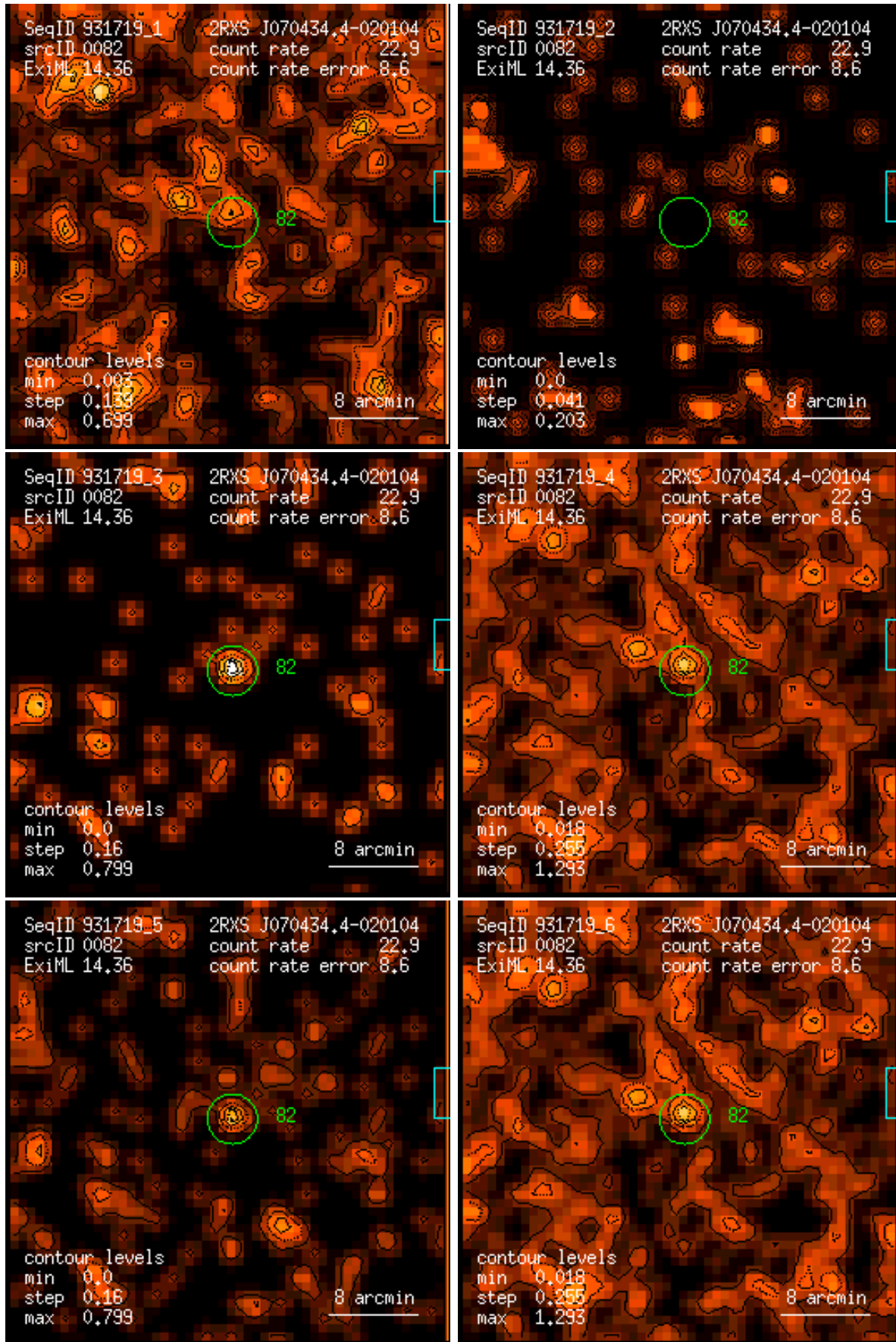
Figure 82: RASS 931719: detection 0082: band rate images, Gaussian filter: (1) PSPC channels 11 – 41, (2) 52 – 90, (3) 91 – 201, (4) 11 – 235, (5) 52 – 201, (6) 11 – 201. Broad band rates in counts/ks. Band rate contour levels in counts/ks/arcmin 2 .
