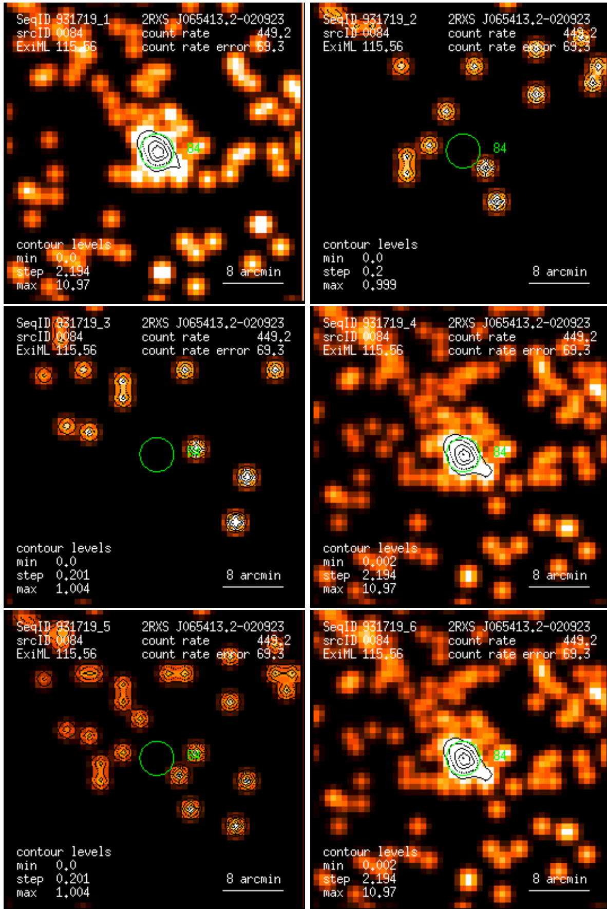
Figure 84: RASS 931719: detection 0084: band rate images, Gaussian filter: (1) PSPC channels 11 – 41, (2) 52 – 90, (3) 91 – 201, (4) 11 – 235, (5) 52 – 201, (6) 11 – 201. Broad band rates in counts/ks. Band rate contour levels in counts/ks/arcmin 2 .
