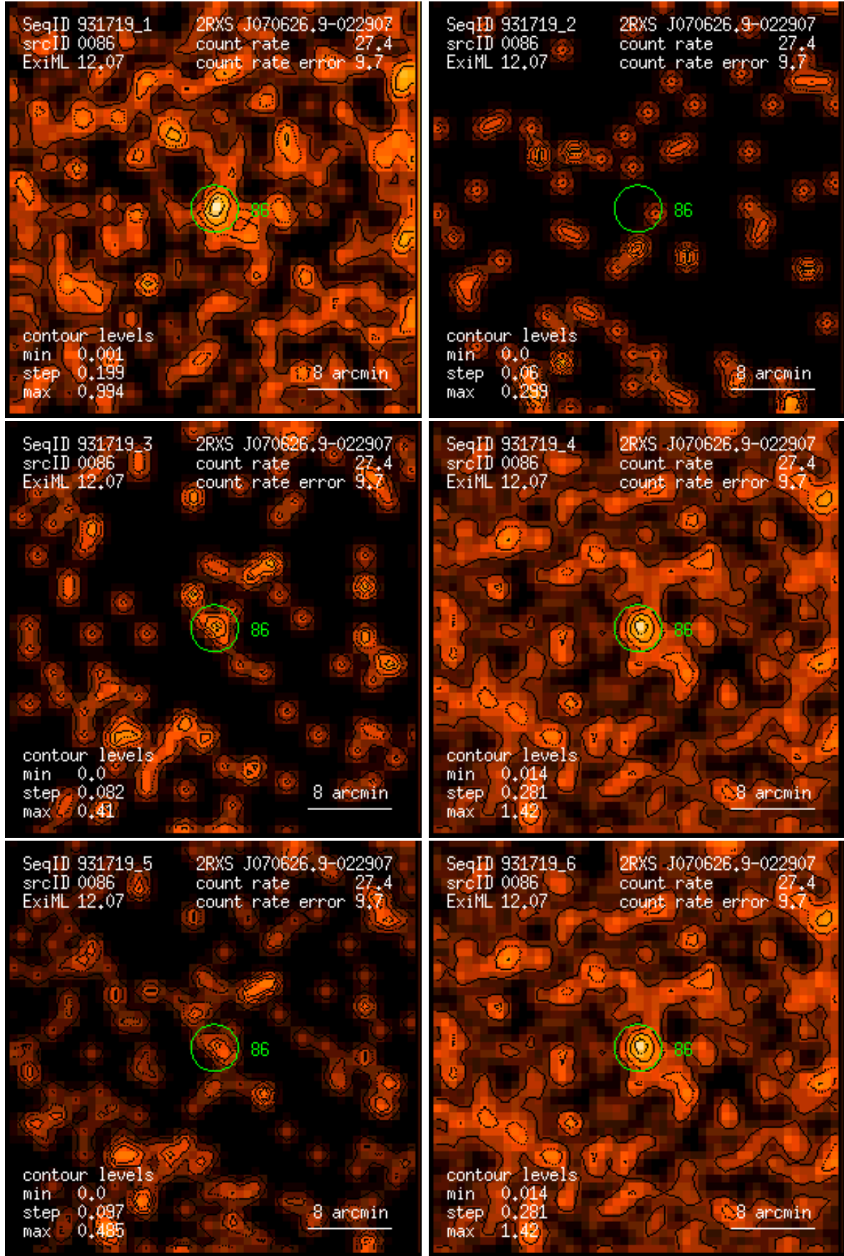
Figure 86: RASS 931719: detection 0086: band rate images, Gaussian filter: (1) PSPC channels 11 – 41, (2) 52 – 90, (3) 91 – 201, (4) 11 – 235, (5) 52 – 201, (6) 11 – 201. Broad band rates in counts/ks. Band rate contour levels in counts/ks/arcmin 2 .
