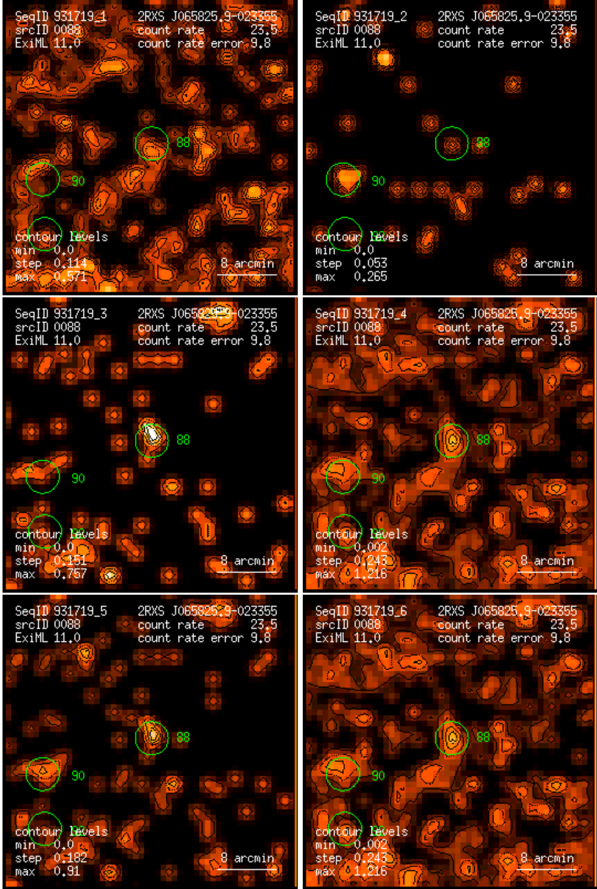
Figure 88: RASS 931719: detection 0088: band rate images, Gaussian filter: (1) PSPC channels 11 – 41, (2) 52 – 90, (3) 91 – 201, (4) 11 – 235, (5) 52 – 201, (6) 11 – 201. Broad band rates in counts/ks. Band rate contour levels in counts/ks/arcmin 2 .
