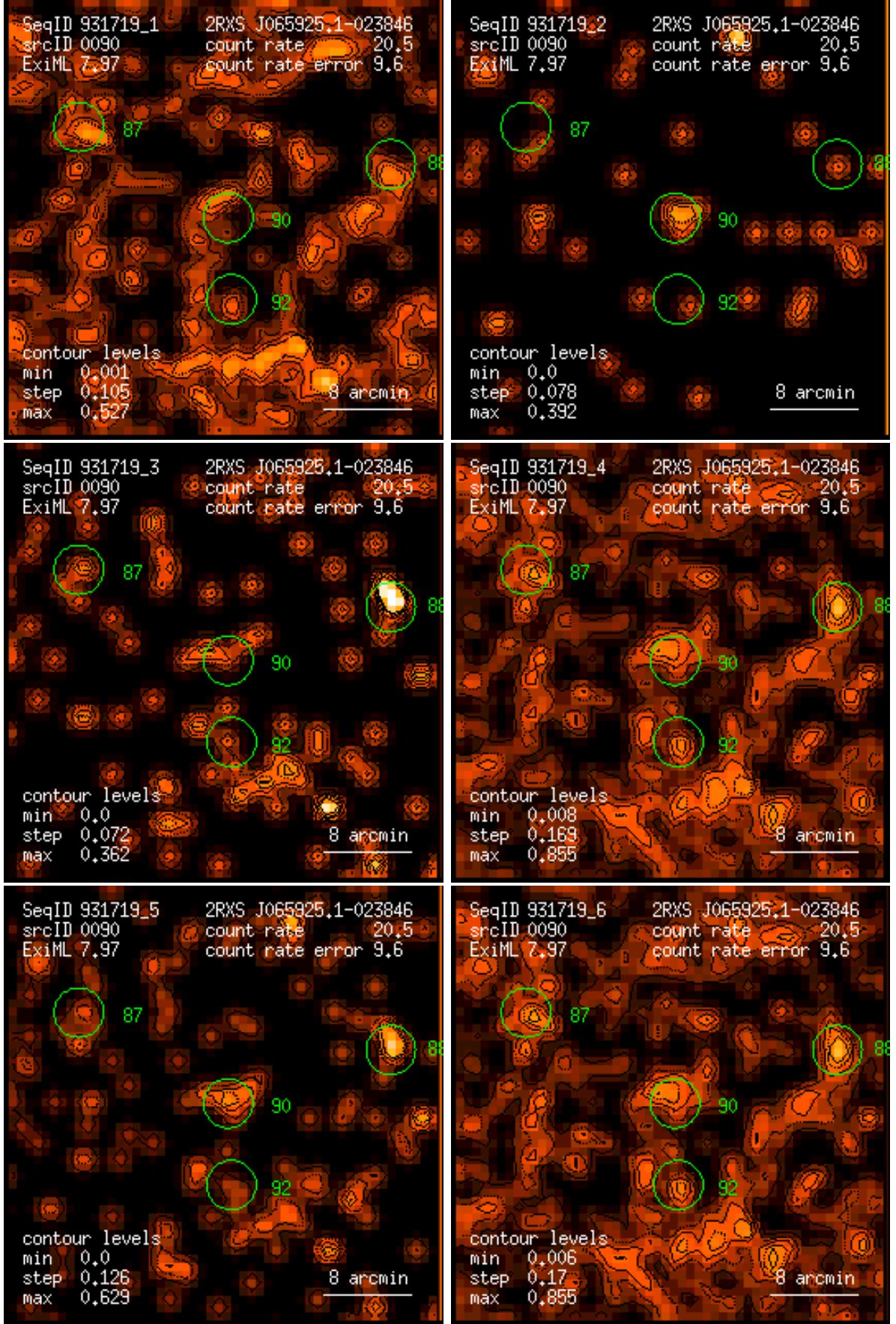
Figure 90: RASS 931719: detection 0090: band rate images, Gaussian filter: (1) PSPC channels 11 – 41, (2) 52 – 90, (3) 91 – 201, (4) 11 – 235, (5) 52 – 201, (6) 11 – 201. Broad band rates in counts/ks. Band rate contour levels in counts/ks/arcmin 2 .
