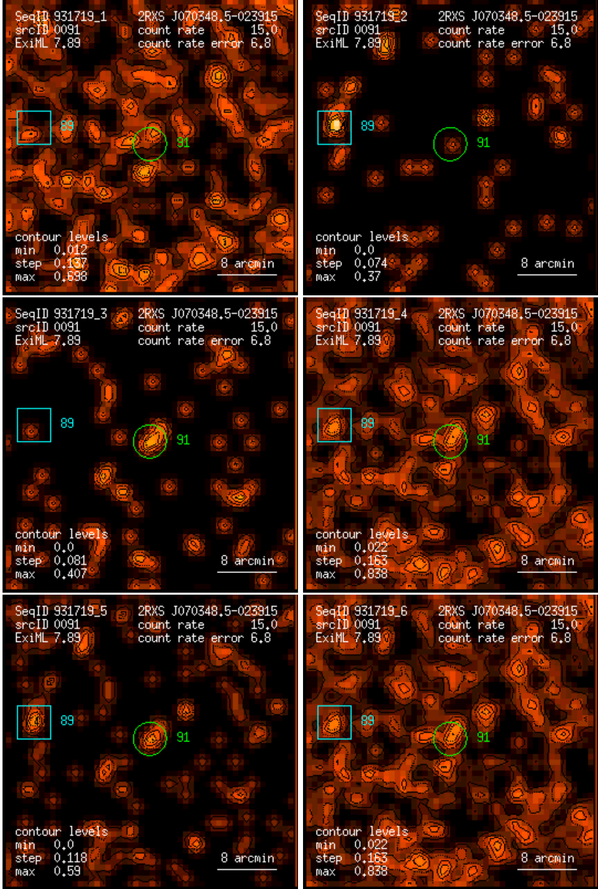
Figure 91: RASS 931719: detection 0091: band rate images, Gaussian filter: (1) PSPC channels 11 – 41, (2) 52 – 90, (3) 91 – 201, (4) 11 – 235, (5) 52 – 201, (6) 11 – 201. Broad band rates in counts/ks. Band rate contour levels in counts/ks/arcmin 2 .
