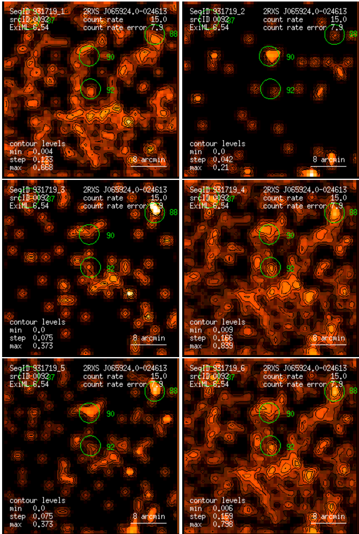
Figure 92: RASS 931719: detection 0092: band rate images, Gaussian filter: (1) PSPC channels 11 – 41, (2) 52 – 90, (3) 91 – 201, (4) 11 – 235, (5) 52 – 201, (6) 11 – 201. Broad band rates in counts/ks. Band rate contour levels in counts/ks/arcmin 2 .
