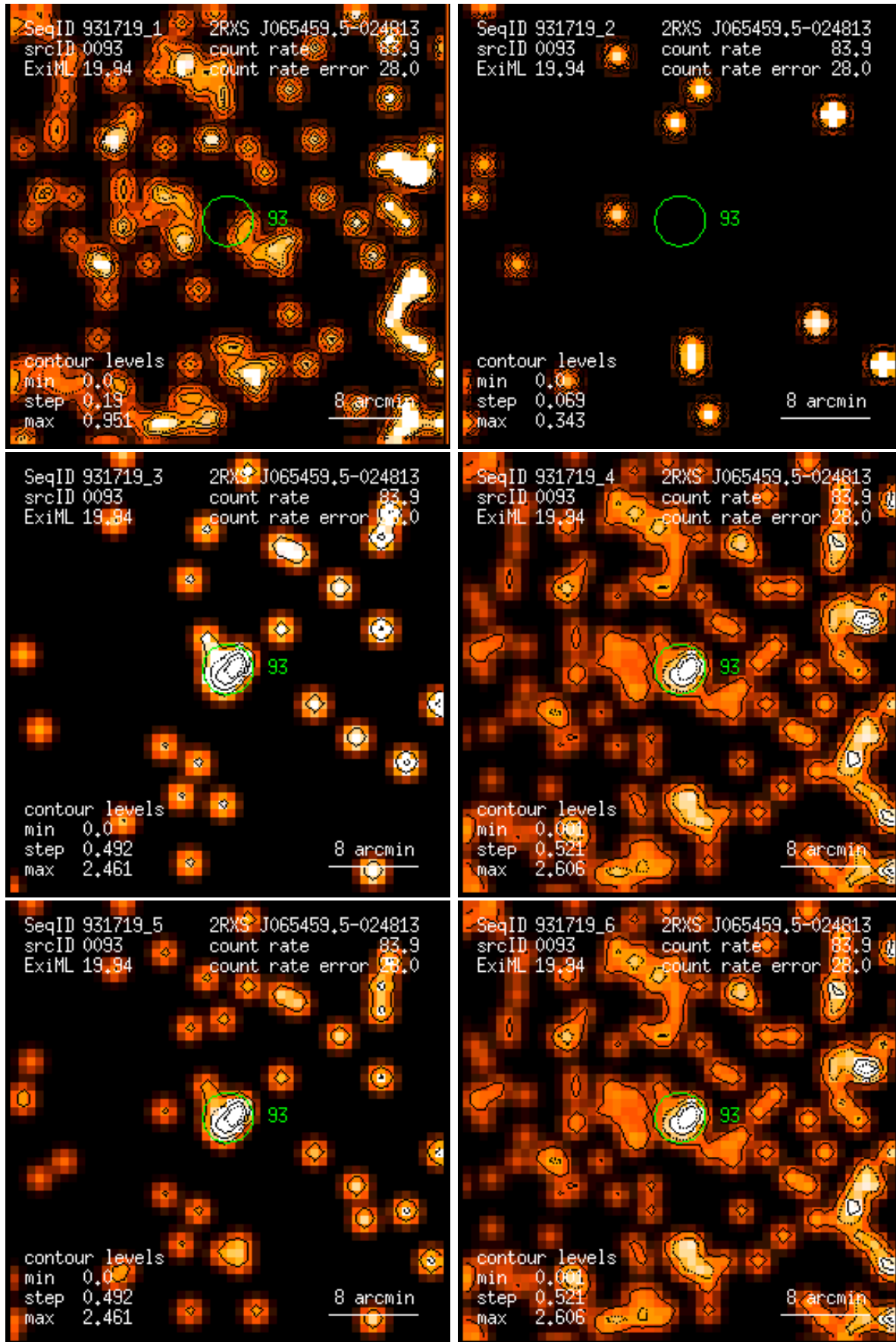
Figure 93: RASS 931719: detection 0093: band rate images, Gaussian filter: (1) PSPC channels 11 – 41, (2) 52 – 90, (3) 91 – 201, (4) 11 – 235, (5) 52 – 201, (6) 11 – 201. Broad band rates in counts/ks. Band rate contour levels in counts/ks/arcmin 2 .
