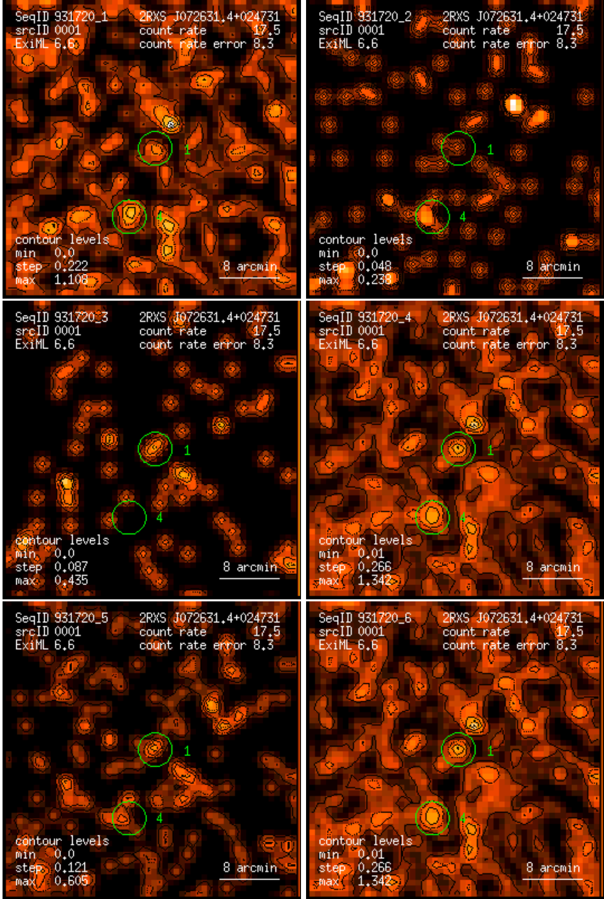
Figure 1: RASS 931720: detection 0001: band rate images, Gaussian filter: (1) PSPC channels 11 – 41, (2) 52 – 90, (3) 91 – 201, (4) 11 – 235, (5) 52 – 201, (6) 11 – 201. Broad band rates in counts/ks. Band rate contour levels in counts/ks/arcmin 2 .
