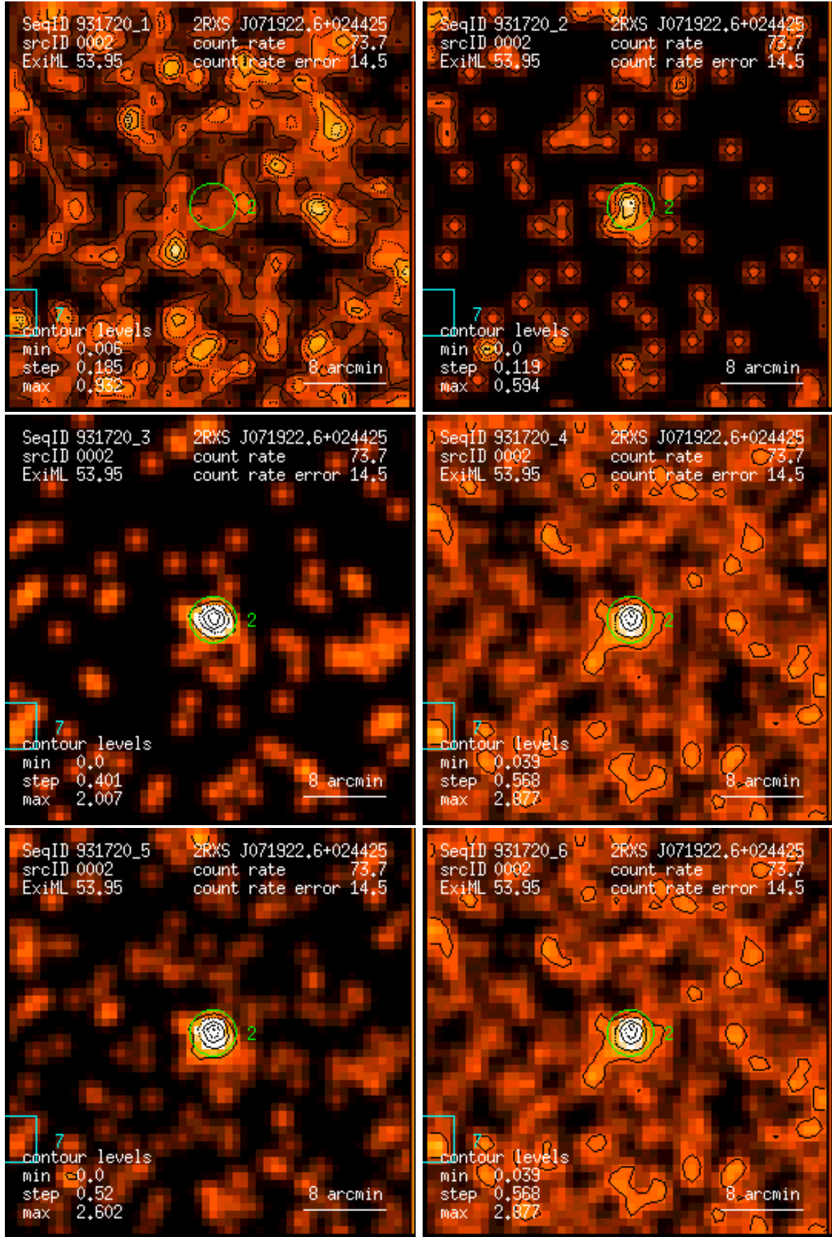
Figure 2: RASS 931720: detection 0002: band rate images, Gaussian filter: (1) PSPC channels 11 – 41, (2) 52 – 90, (3) 91 – 201, (4) 11 – 235, (5) 52 – 201, (6) 11 – 201. Broad band rates in counts/ks. Band rate contour levels in counts/ks/arcmin 2 .
