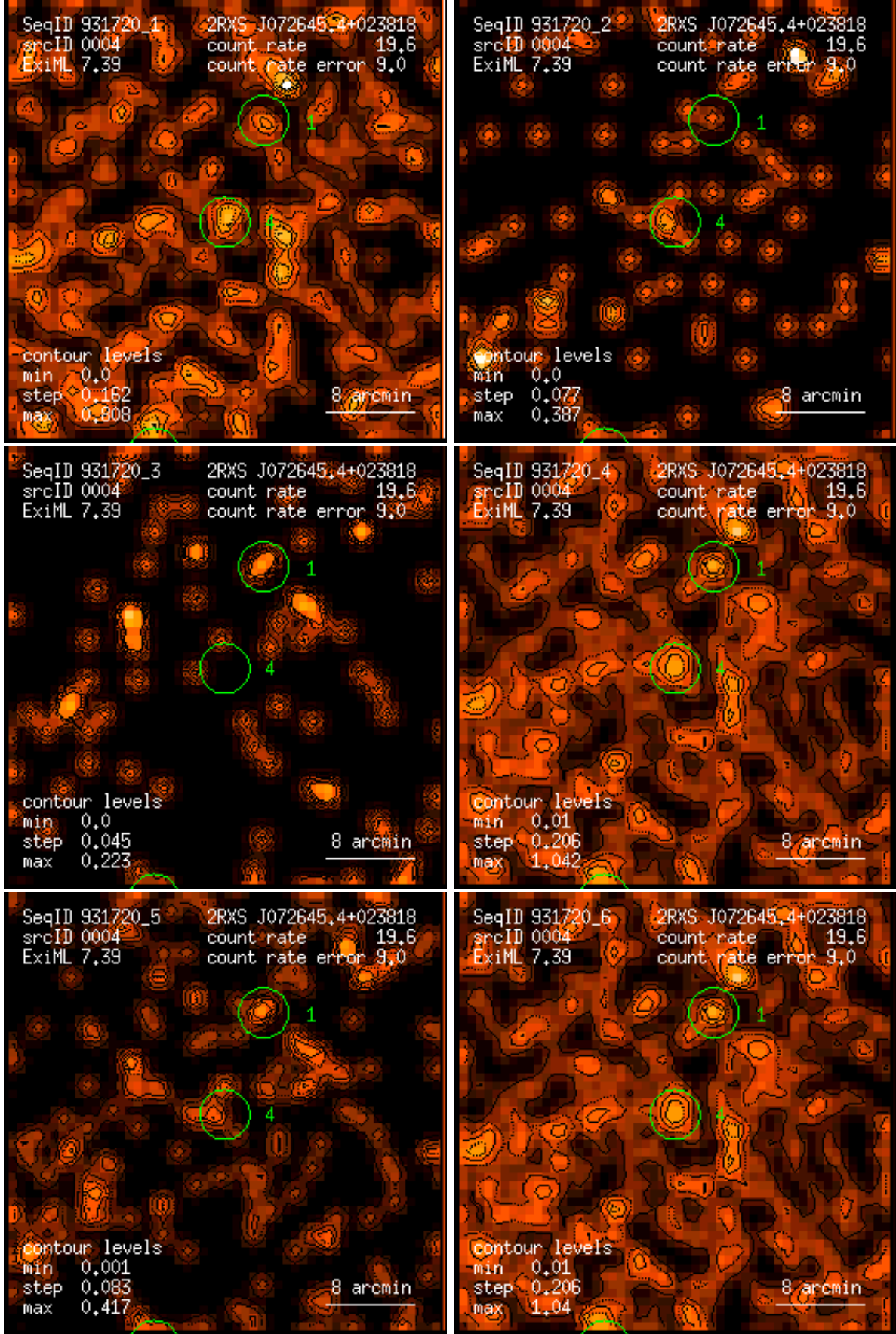
Figure 4: RASS 931720: detection 0004: band rate images, Gaussian filter: (1) PSPC channels 11 – 41, (2) 52 – 90, (3) 91 – 201, (4) 11 – 235, (5) 52 – 201, (6) 11 – 201. Broad band rates in counts/ks. Band rate contour levels in counts/ks/arcmin 2 .
