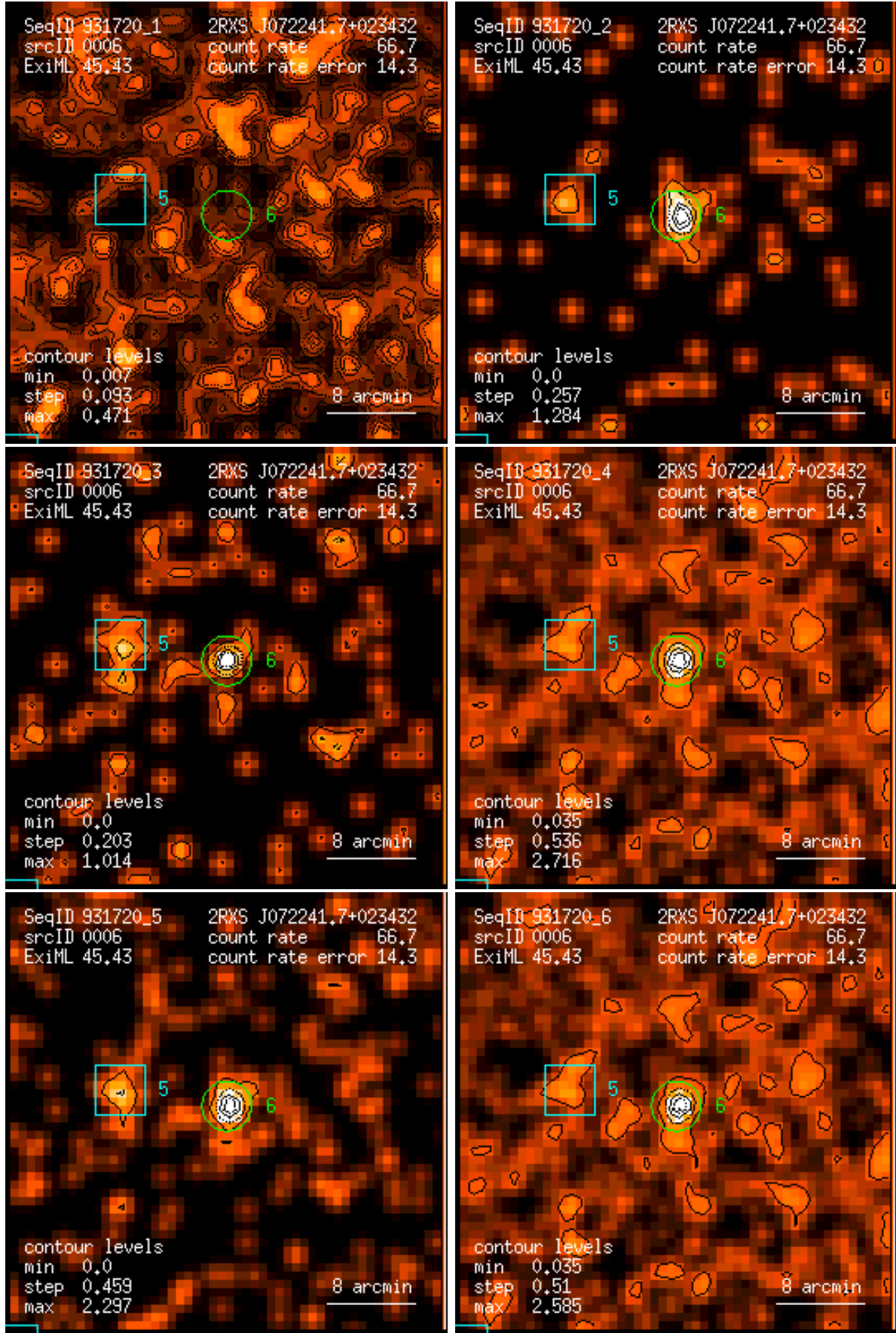
Figure 6: RASS 931720: detection 0006: band rate images, Gaussian filter: (1) PSPC channels 11 – 41, (2) 52 – 90, (3) 91 – 201, (4) 11 – 235, (5) 52 – 201, (6) 11 – 201. Broad band rates in counts/ks. Band rate contour levels in counts/ks/arcmin 2 .
