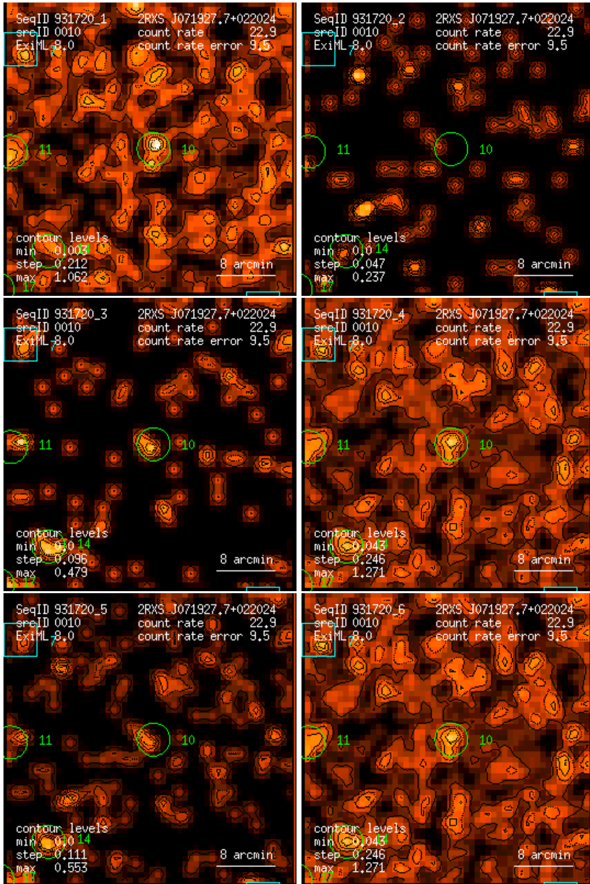
Figure 10: RASS 931720: detection 0010: band rate images, Gaussian filter: (1) PSPC channels 11 – 41, (2) 52 – 90, (3) 91 – 201, (4) 11 – 235, (5) 52 – 201, (6) 11 – 201. Broad band rates in counts/ks. Band rate contour levels in counts/ks/arcmin 2 .
