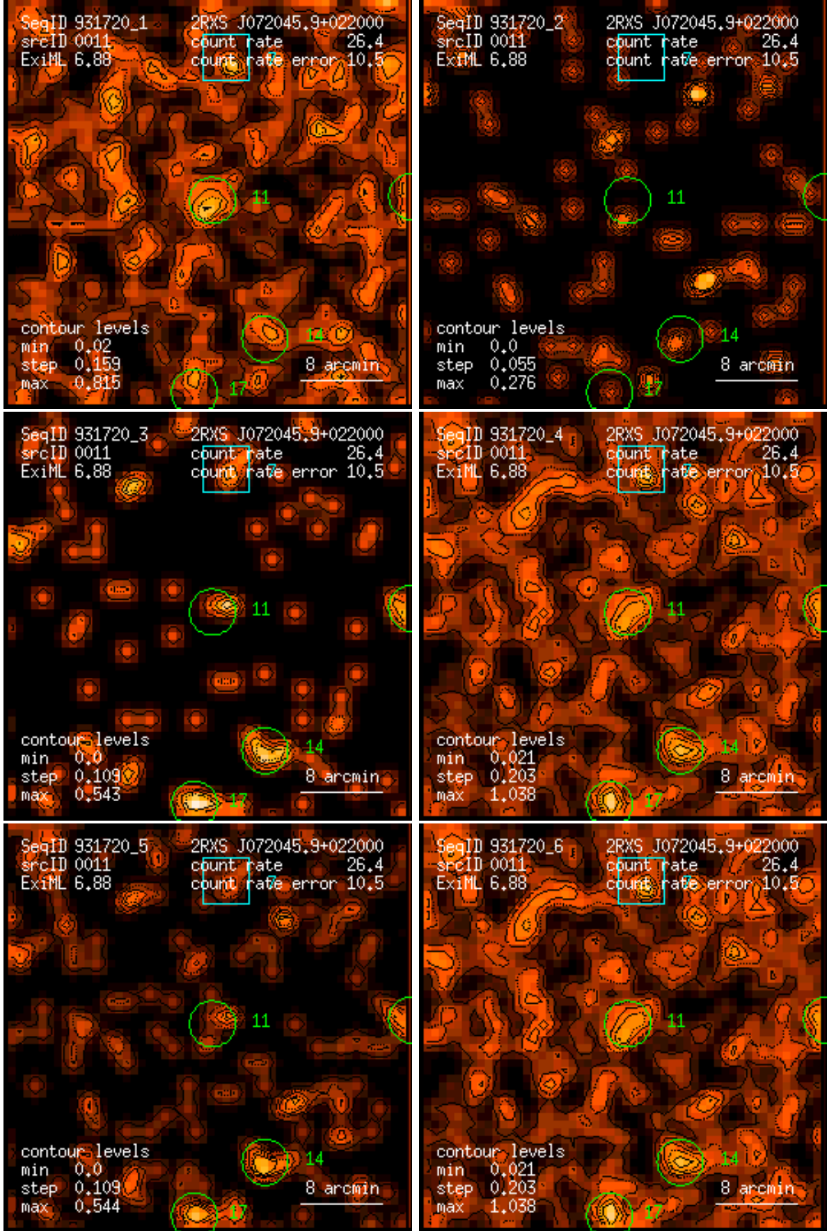
Figure 11: RASS 931720: detection 0011: band rate images, Gaussian filter: (1) PSPC channels 11 – 41, (2) 52 – 90, (3) 91 – 201, (4) 11 – 235, (5) 52 – 201, (6) 11 – 201. Broad band rates in counts/ks. Band rate contour levels in counts/ks/arcmin 2 .
