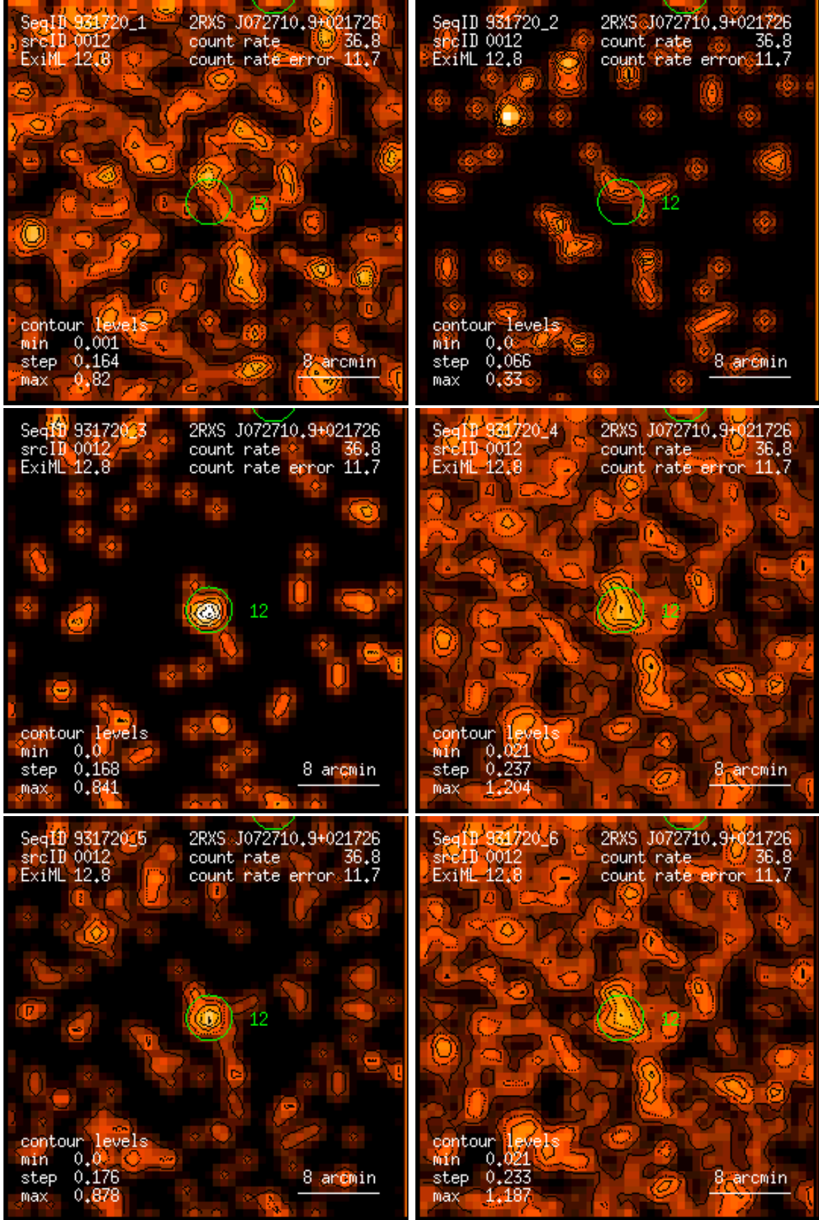
Figure 12: RASS 931720: detection 0012: band rate images, Gaussian filter: (1) PSPC channels 11 – 41, (2) 52 – 90, (3) 91 – 201, (4) 11 – 235, (5) 52 – 201, (6) 11 – 201. Broad band rates in counts/ks. Band rate contour levels in counts/ks/arcmin 2 .
