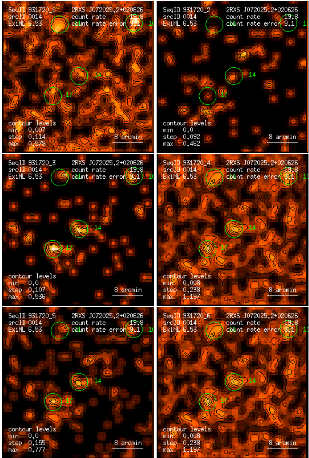
Figure 14: RASS 931720: detection 0014: band rate images, Gaussian filter: (1) PSPC channels 11 – 41, (2) 52 – 90, (3) 91 – 201, (4) 11 – 235, (5) 52 – 201, (6) 11 – 201. Broad band rates in counts/ks. Band rate contour levels in counts/ks/arcmin 2 .
