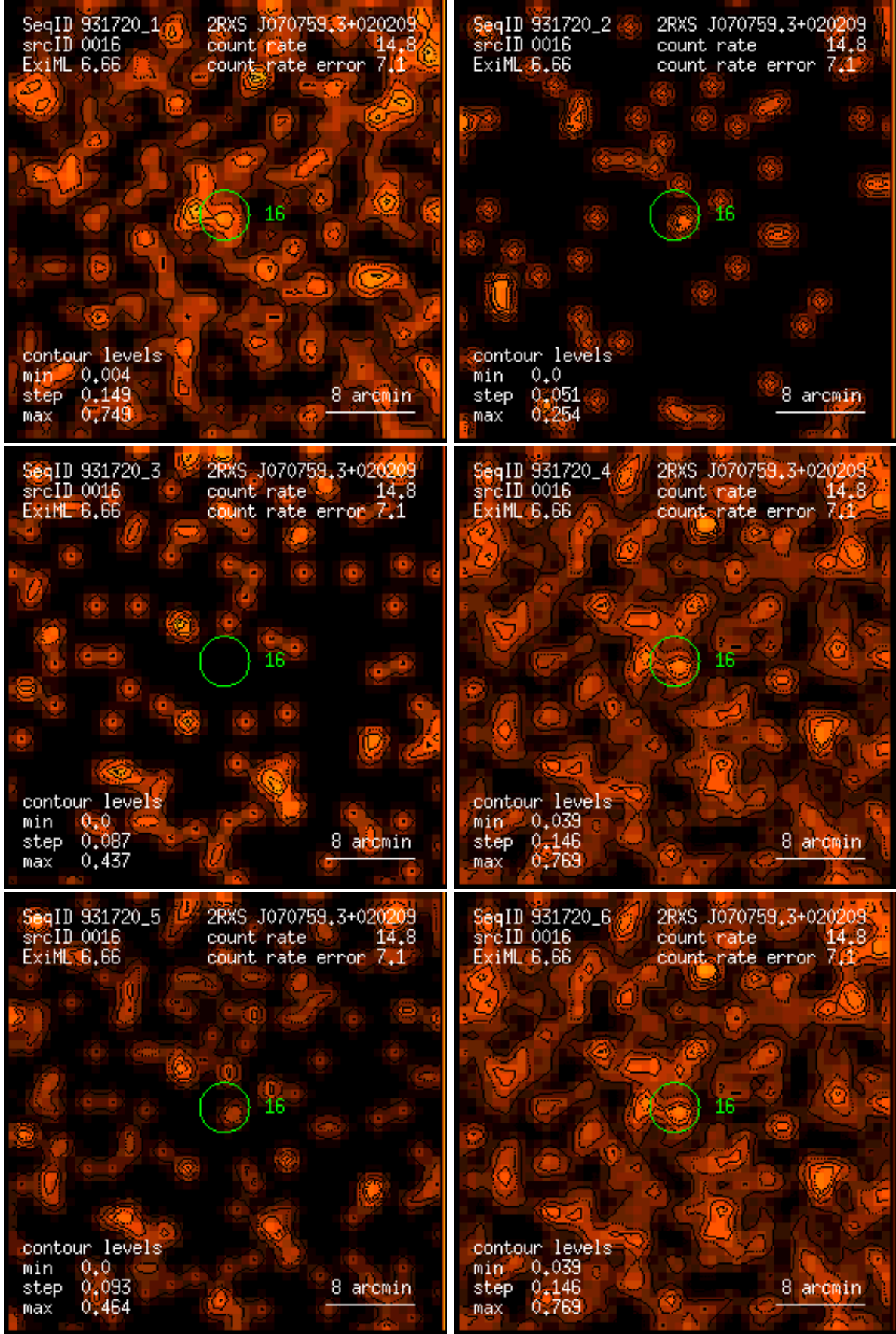
Figure 16: RASS 931720: detection 0016: band rate images, Gaussian filter: (1) PSPC channels 11 – 41, (2) 52 – 90, (3) 91 – 201, (4) 11 – 235, (5) 52 – 201, (6) 11 – 201. Broad band rates in counts/ks. Band rate contour levels in counts/ks/arcmin 2 .
