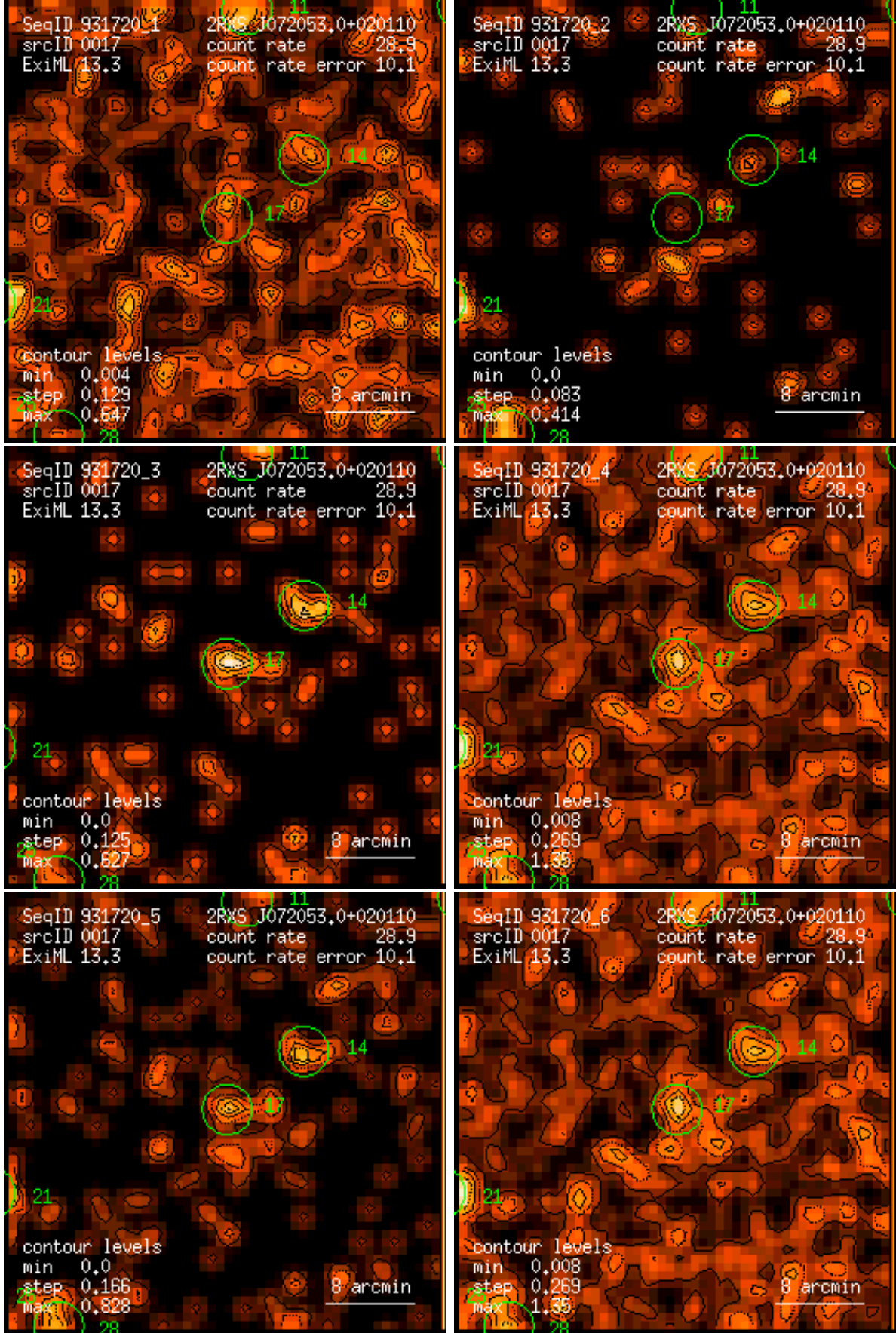
Figure 17: RASS 931720: detection 0017: band rate images, Gaussian filter: (1) PSPC channels 11 – 41, (2) 52 – 90, (3) 91 – 201, (4) 11 – 235, (5) 52 – 201, (6) 11 – 201. Broad band rates in counts/ks. Band rate contour levels in counts/ks/arcmin 2 .
