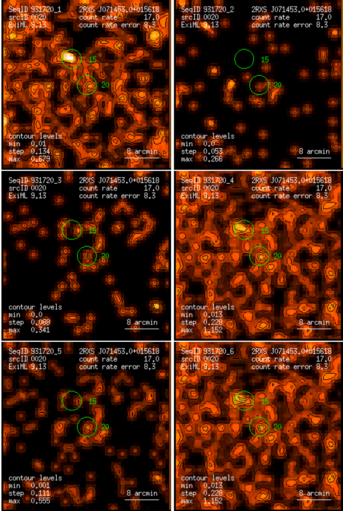
Figure 20: RASS 931720: detection 0020: band rate images, Gaussian filter: (1) PSPC channels 11 – 41, (2) 52 – 90, (3) 91 – 201, (4) 11 – 235, (5) 52 – 201, (6) 11 – 201. Broad band rates in counts/ks. Band rate contour levels in counts/ks/arcmin 2 .
