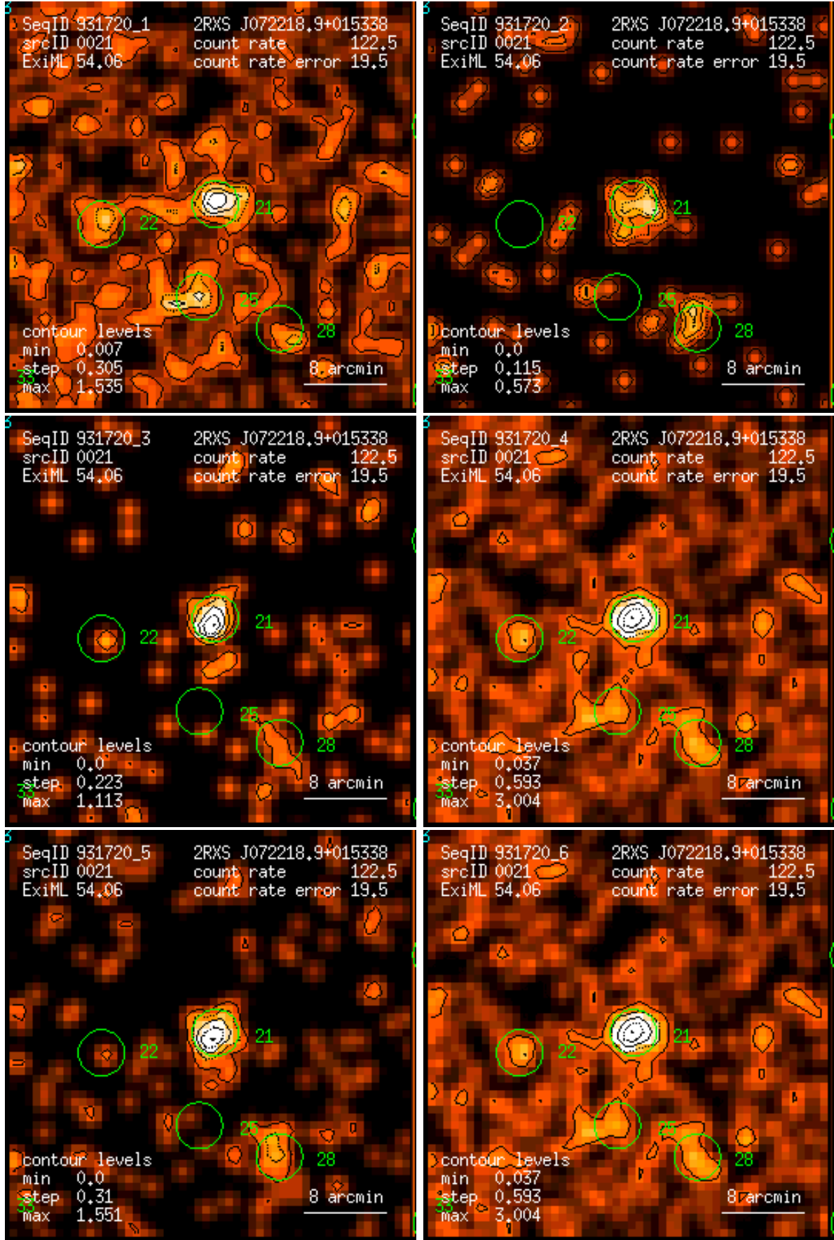
Figure 21: RASS 931720: detection 0021: band rate images, Gaussian filter: (1) PSPC channels 11 – 41, (2) 52 – 90, (3) 91 – 201, (4) 11 – 235, (5) 52 – 201, (6) 11 – 201. Broad band rates in counts/ks. Band rate contour levels in counts/ks/arcmin 2 .
