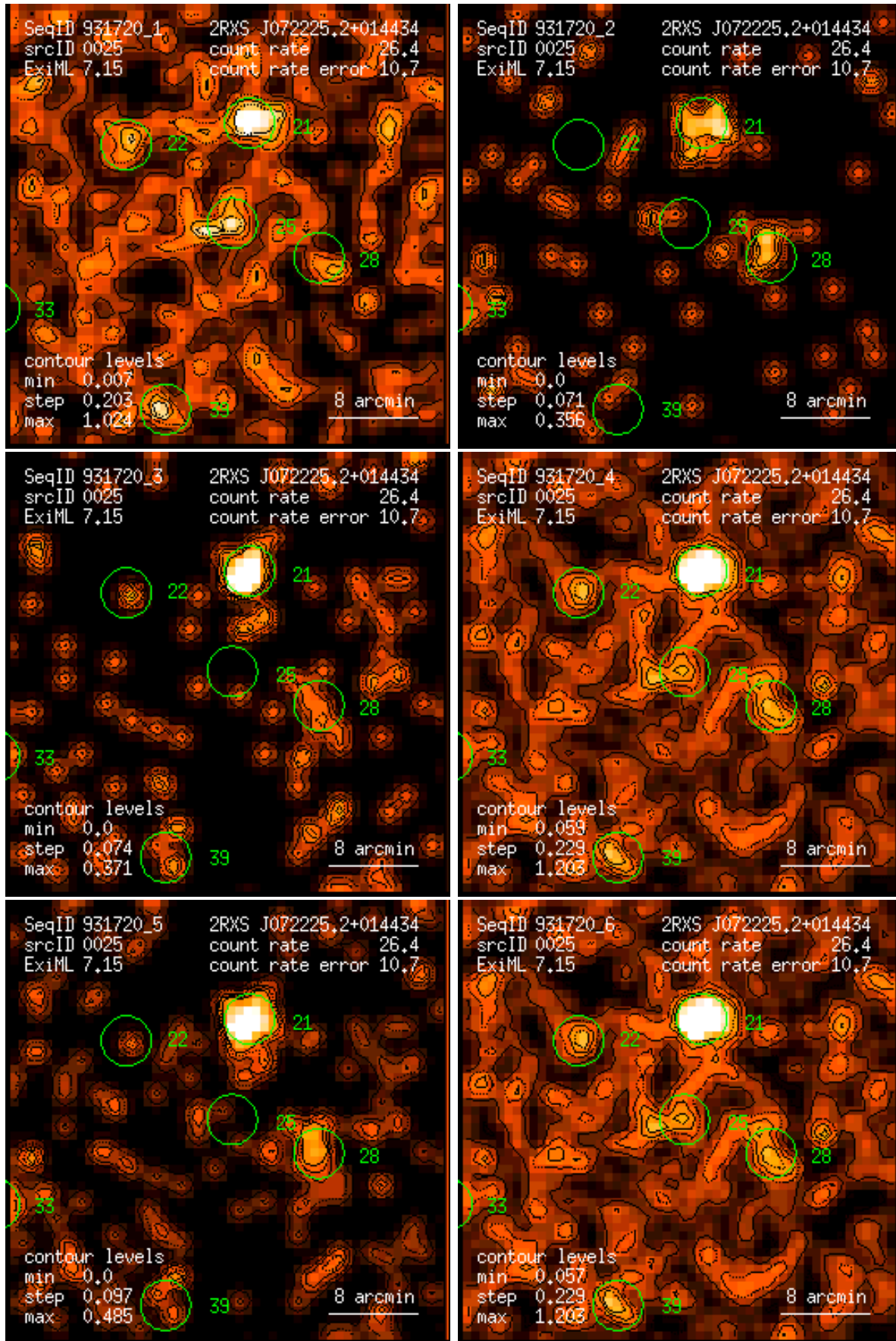
Figure 25: RASS 931720: detection 0025: band rate images, Gaussian filter: (1) PSPC channels 11 – 41, (2) 52 – 90, (3) 91 – 201, (4) 11 – 235, (5) 52 – 201, (6) 11 – 201. Broad band rates in counts/ks. Band rate contour levels in counts/ks/arcmin 2 .
