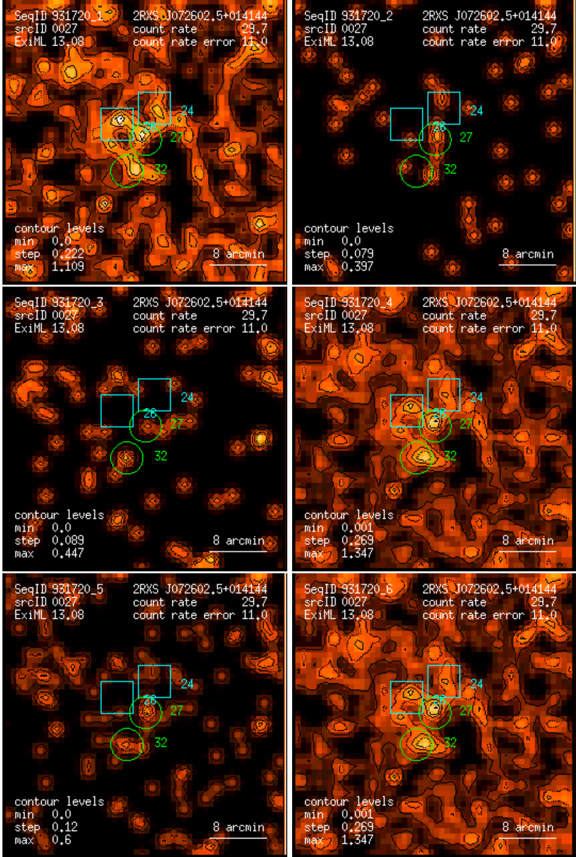
Figure 27: RASS 931720: detection 0027: band rate images, Gaussian filter: (1) PSPC channels 11 – 41, (2) 52 – 90, (3) 91 – 201, (4) 11 – 235, (5) 52 – 201, (6) 11 – 201. Broad band rates in counts/ks. Band rate contour levels in counts/ks/arcmin 2 .
