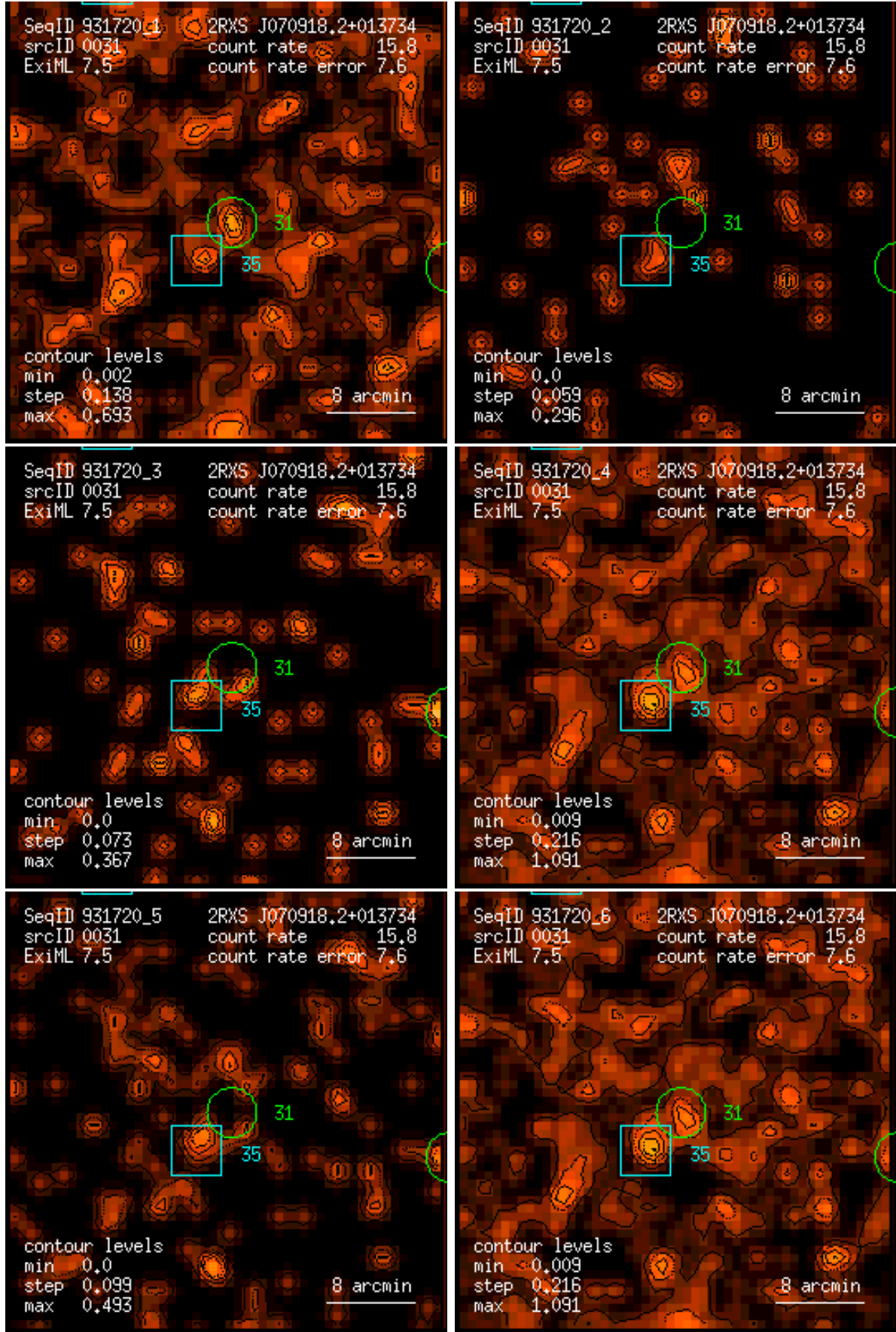
Figure 31: RASS 931720: detection 0031: band rate images, Gaussian filter: (1) PSPC channels 11 – 41, (2) 52 – 90, (3) 91 – 201, (4) 11 – 235, (5) 52 – 201, (6) 11 – 201. Broad band rates in counts/ks. Band rate contour levels in counts/ks/arcmin 2 .
