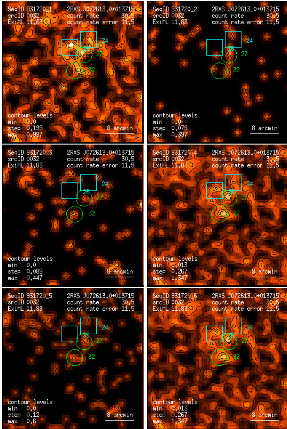
Figure 32: RASS 931720: detection 0032: band rate images, Gaussian filter: (1) PSPC channels 11 – 41, (2) 52 – 90, (3) 91 – 201, (4) 11 – 235, (5) 52 – 201, (6) 11 – 201. Broad band rates in counts/ks. Band rate contour levels in counts/ks/arcmin 2 .
