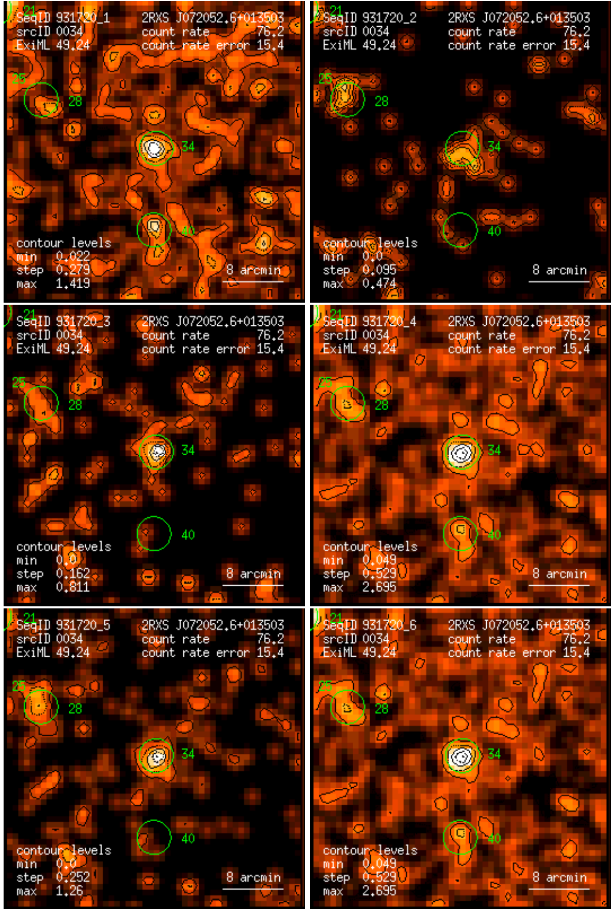
Figure 34: RASS 931720: detection 0034: band rate images, Gaussian filter: (1) PSPC channels 11 – 41, (2) 52 – 90, (3) 91 – 201, (4) 11 – 235, (5) 52 – 201, (6) 11 – 201. Broad band rates in counts/ks. Band rate contour levels in counts/ks/arcmin 2 .
