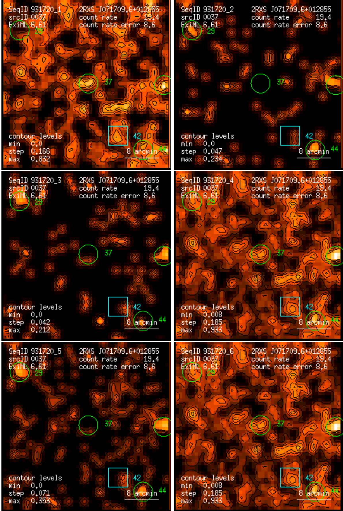
Figure 37: RASS 931720: detection 0037: band rate images, Gaussian filter: (1) PSPC channels 11 – 41, (2) 52 – 90, (3) 91 – 201, (4) 11 – 235, (5) 52 – 201, (6) 11 – 201. Broad band rates in counts/ks. Band rate contour levels in counts/ks/arcmin 2 .
