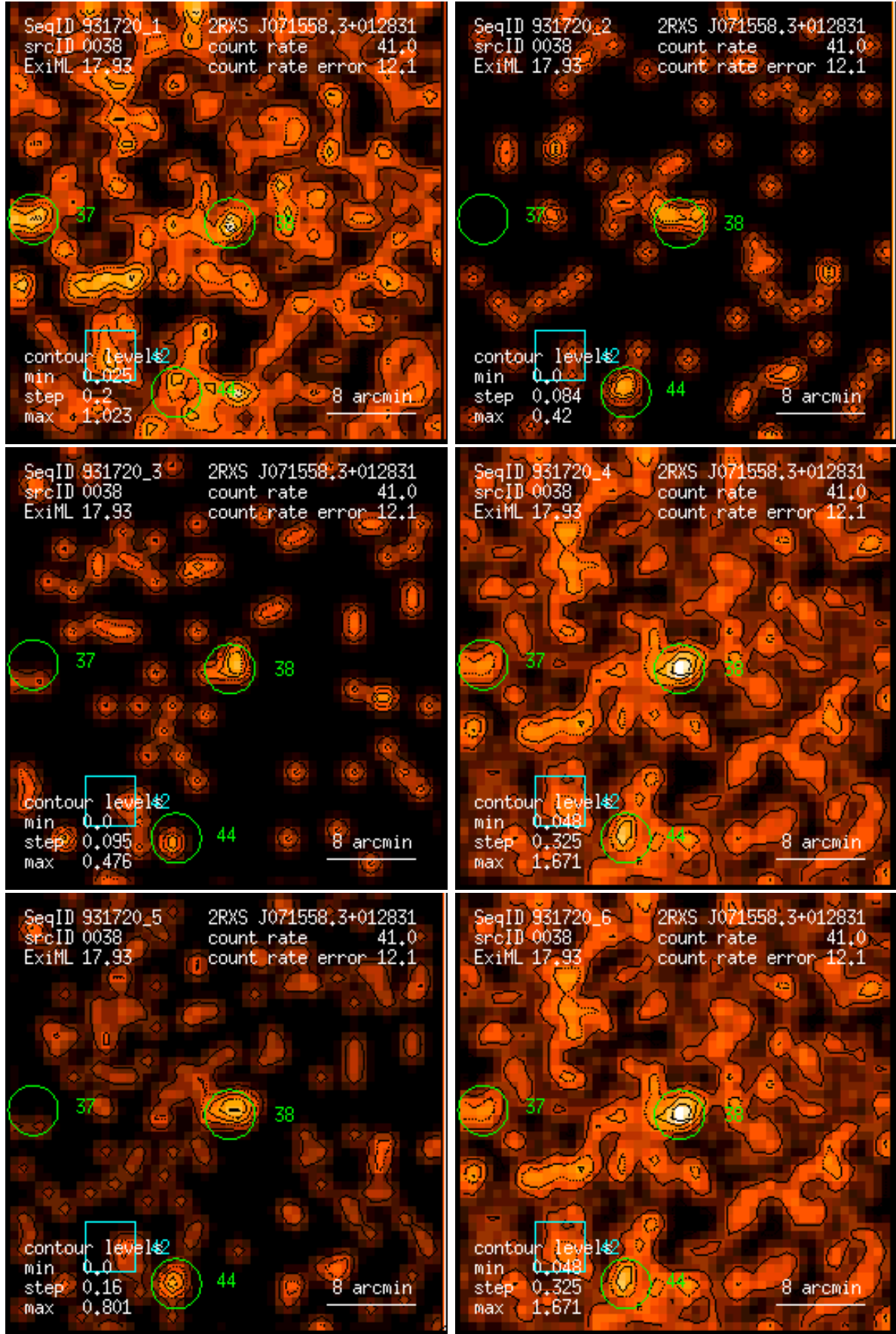
Figure 38: RASS 931720: detection 0038: band rate images, Gaussian filter: (1) PSPC channels 11 – 41, (2) 52 – 90, (3) 91 – 201, (4) 11 – 235, (5) 52 – 201, (6) 11 – 201. Broad band rates in counts/ks. Band rate contour levels in counts/ks/arcmin 2 .
