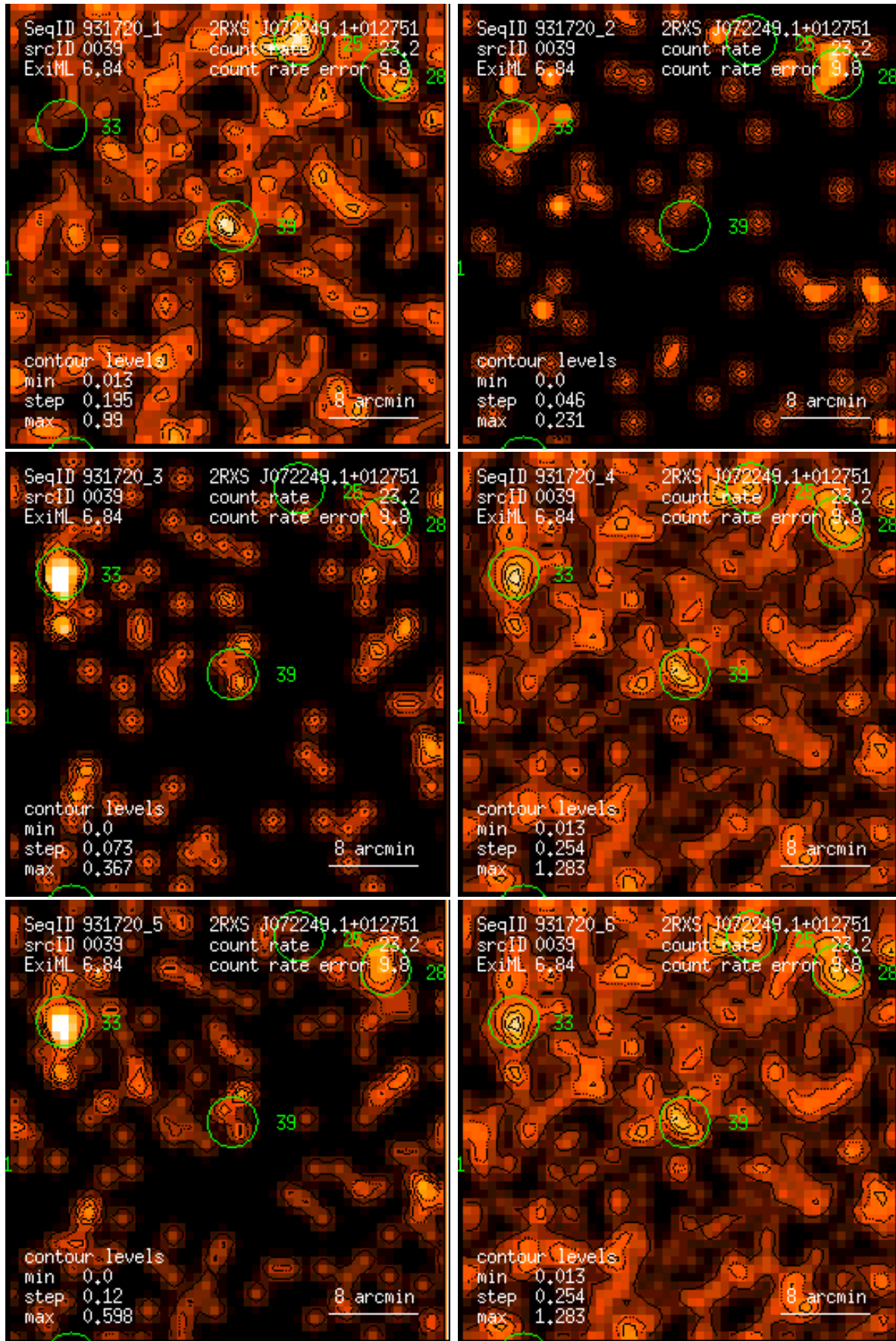
Figure 39: RASS 931720: detection 0039: band rate images, Gaussian filter: (1) PSPC channels 11 – 41, (2) 52 – 90, (3) 91 – 201, (4) 11 – 235, (5) 52 – 201, (6) 11 – 201. Broad band rates in counts/ks. Band rate contour levels in counts/ks/arcmin 2 .
