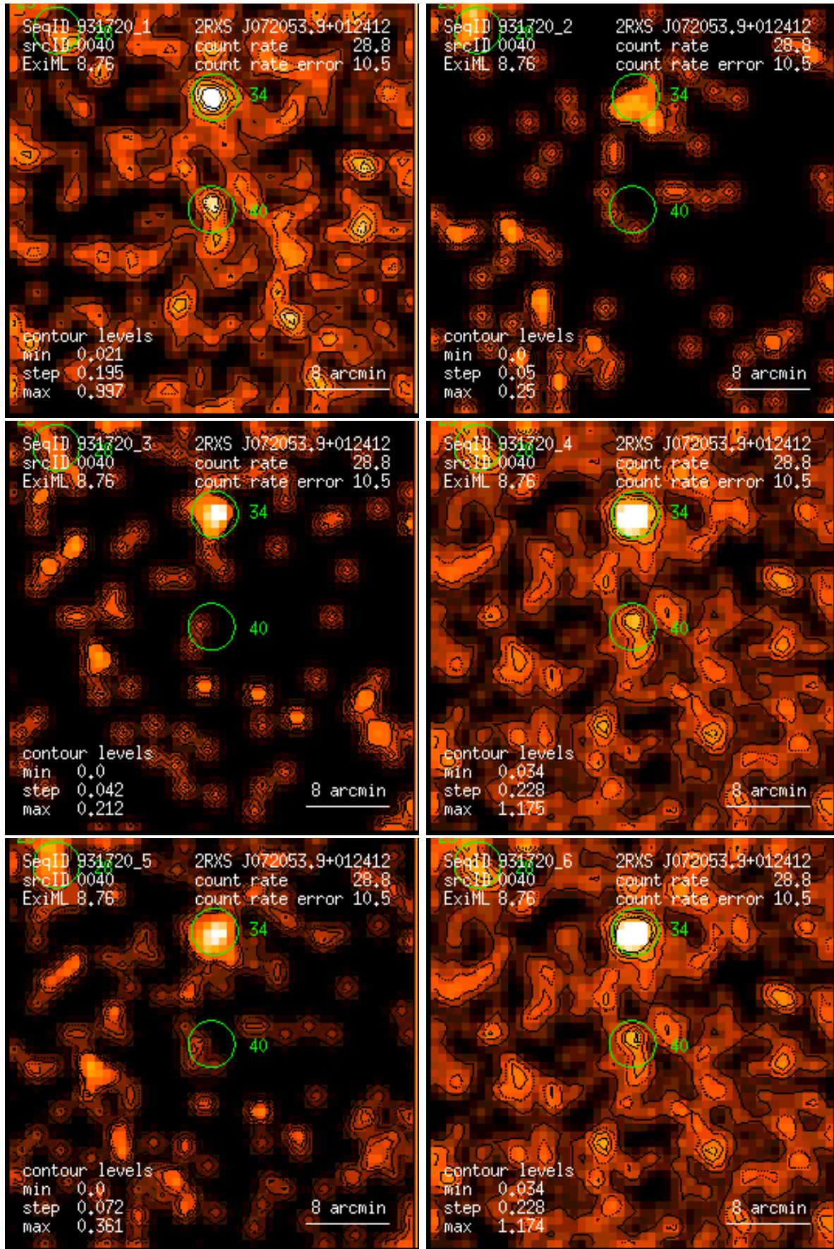
Figure 40: RASS 931720: detection 0040: band rate images, Gaussian filter: (1) PSPC channels 11 – 41, (2) 52 – 90, (3) 91 – 201, (4) 11 – 235, (5) 52 – 201, (6) 11 – 201. Broad band rates in counts/ks. Band rate contour levels in counts/ks/arcmin 2 .
